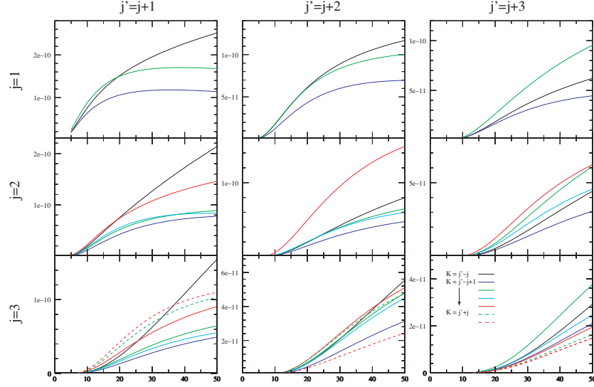
Figure 2. Averaged opacity tensors \langle \pi/k^2 P_{jj'}^K \rangle_T as a function of temperature (in K). They do not decrease with K and their relative magnitude vary with temperature.
