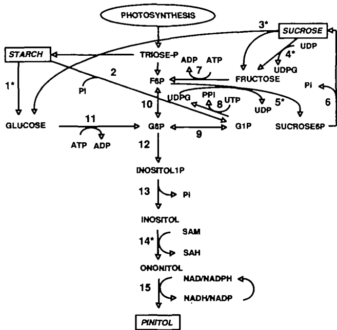
FIG. 1. Simplified scheme depicting the partitioning of carbon between starch, sucrose and pinitol in pigeonpea leaves. Enzymes: 1, total amyolytic activity; 2, starch phosphorylase; 3, invertase; 4, sucrose synthase; 5, sucrose phosphate synthase; 6, sucrose phosphate phosphatase; 7, fructokinase; 8, UDPG-pyrophosphorylase; 9, glucose phosphate mutase; 10, glucose phosphate isomerase; 11, glucokinase; 12, myo -inositol 1-phosphate synthase; 13, myo -inositol phosphate phosphatase; 14, myo -inositol O -methyl transferase; 15, pinitol epimerase. Metabolites: G1P, glucose 1-phosphate; G6P, glucose 6-phosphate; F6P, fructose 6-phosphate; SAM, S -adenosyl-L-methionine; SAH, S -adenosyl-L-homocysteine. Enzymes marked with an asterisk were measured in this study.
