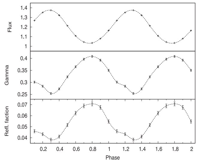
Figure 14. Best-fitting parameters 1\sigma errors for the 10 phase-resolved spectra. From top to bottom: RELXILL 0.5–10 keV unabsorbed flux in units of 10^{-8} \text{ erg cm}^{-2} \text{ s}^{-1} , photon index and reflection fraction.
