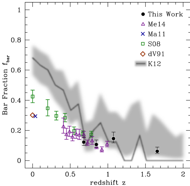
Figure 6. Fraction of disc galaxies having a strong bar feature versus redshift, in the context of other work assessing visual strong bar fraction. All shading and error bars indicate 1\sigma Bayesian binomial confidence intervals (Cameron 2011); where necessary, we have re-calculated uncertainties of other studies so that all uncertainties shown here are based on the same method. Error bars for the Masters et al. (2011, Ma11, blue cross) and de Vaucouleurs et al. (1991, dV91, red diamond) fractions are smaller than the size of the points and are omitted. At higher redshift, bar fractions in this work (black circles) at z < 1 are consistent with those of Sheth et al. (2008, S08, green squares) and Melvin et al. (2014, Me14, purple triangles) despite differences in selection methods and including our conservative completeness correction. Kraljic et al. (2012, K12) computed the fraction of strong bars to z = 2 among modelled disc galaxies that evolved to stellar masses M_* \approx 10^{10-11} M_\odot (shaded region); the predicted bar fraction is consistent with that observed here within the uncertainties, although we note that the differences between simulated and observed mass/luminosity ranges make direct quantitative comparisons more difficult.
