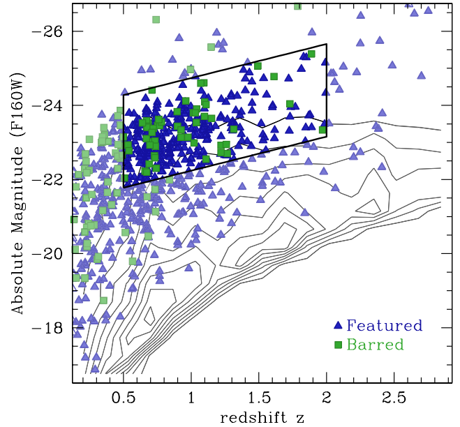
Figure 4. Absolute H -band magnitude versus redshift for all sources with H < 25.5 (contours in steps of 10 per cent) and 876 discs (DISC-PARENT sample; blue triangles), of which 123 galaxies show clear evidence of a bar (BAR-PARENT sample; green squares). To facilitate comparison between lookback times, avoid biases due to surface-brightness dimming when calculating bar fractions, and ensure all observed H -band flux is redwards of the 4000 \text{ \AA} break, we select subsamples within the same region of the evolving galaxy luminosity function (Marchesini et al. 2012) and 0.5 \leq z \leq 2 (parallelogram). Within this region there are 370 disc galaxies (DISC-LZ sample), 56 of which have clear evidence of bars (BAR-LZ sample).
