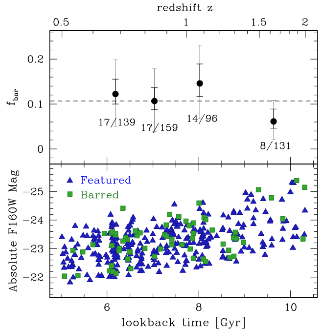
Figure 5. Top panel: bar fraction versus lookback time (black circles) for the completeness-corrected DISC-LZ sample. Black error bars are 68 per cent Bayesian binomial confidence intervals (Cameron 2011); grey error bars are 1\sigma uncertainties combining the binomial confidence intervals with uncertainties due to photometric redshift measurement error and classification error (described in Section 2.5). Within the uncertainties, the bar fraction is consistent with no evolution from 0.5 \leq z \leq 2 . Bins were chosen to enclose similar lookback time intervals; the bar fraction across all bins ( 10.7_{-3.5}^{+6.3} per cent, combined errors) is shown as a dashed line. Bottom panel: absolute H -band magnitudes of the featured disc sample from which the fractions are drawn.
