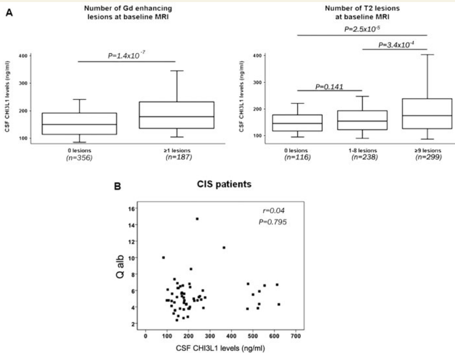
Figure 4 Association between CSF CHI3L1 levels and MRI abnormalities and CSF characteristics. (A) Boxplots showing age-adjusted CSF CHI3L1 levels in CIS patients stratified according to the presence of gadolinium (Gd) enhancing lesions ( left ) and number of T 2 lesions ( right ) at baseline. The number of Gd enhancing lesions was recorded into two categories: 0 lesions / 1 or more lesions. The number of T 2 lesions was recorded into three different categories: 0 lesions / 1–8 lesions / 9 or more lesions. Numbers in parentheses indicate individuals available for analysis. Analysis was performed with a Mann-Whitney’s U-test. (B) Relationship between the albumin CSF/serum ratio (Q alb) and CHI3L1 protein levels in CSF. Albumin CSF/serum ratio was analysed in a subgroup of 59 CIS patients (40 patients from the University of Basel, Switzerland; and 19 patients from the University of Ulm, Germany). r = partial correlation coefficient.
