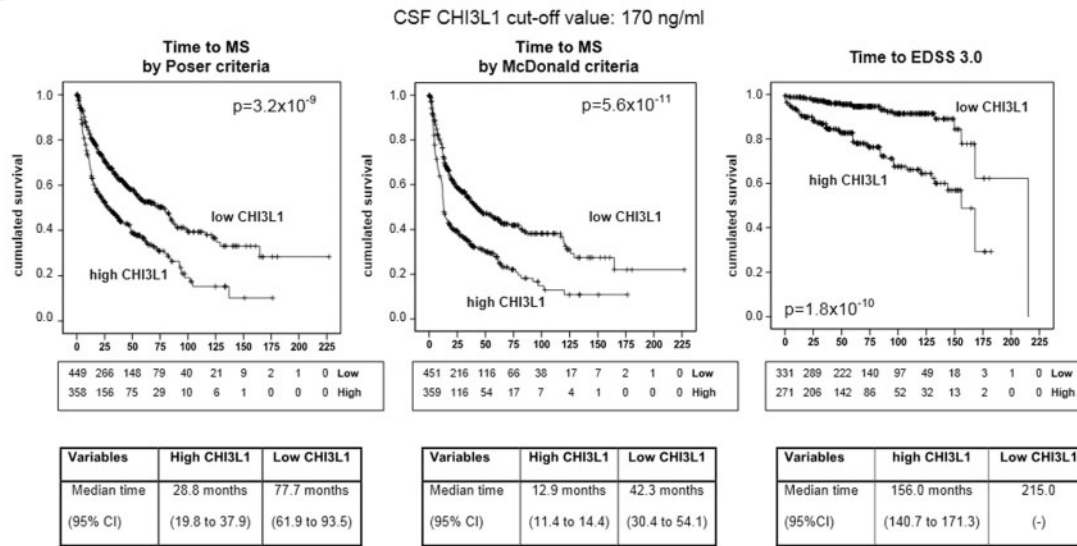
Figure 3 Kaplan-Meier curves for time to multiple sclerosis and time to EDSS 3.0 according to baseline CSF CHI3L1 levels classified into high and low based on a cut-off value of 170 ng/ml. Graphs show log-rank P-values. Numbers represent patients at risk for the different follow-up times. Tables indicate median times (95% CI) to multiple sclerosis and EDSS 3.0 in CIS patients with high and low CHI3L1 levels.
