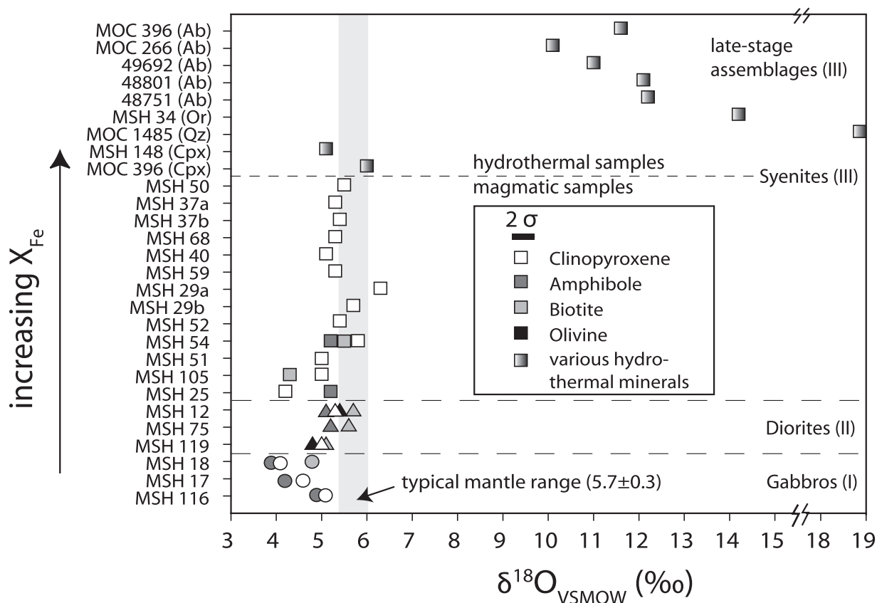
Fig. 12. \delta^{18}\text{O}_{\text{VSMOW}} (‰) data for mineral separates from all units. Fe–Mg silicates are sorted according to increasing X_{\text{Fe}} . Different grey scales represent different minerals; gabbros are represented by circles, diorites by triangles and syenites by squares.
