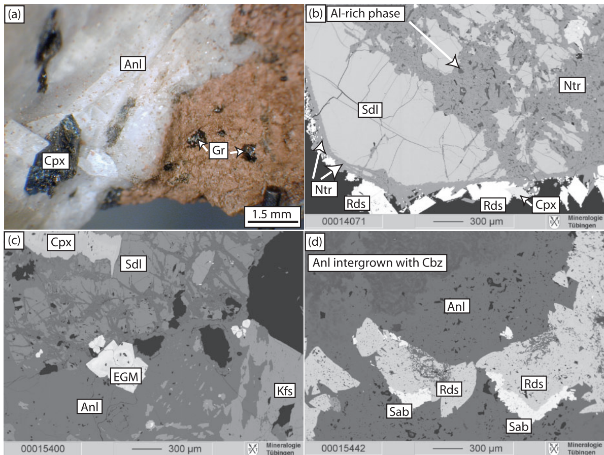
Fig. 3. Textures observed in late-stage assemblages of the foid syenites of Mont Saint-Hilaire. (a) Graphite (Gr) embedded in unidentified matrix surrounding clinopyroxene (Cpx) and analcime (Anl). (b) Relict sodalite (Sdl) rimmed and replaced by natrolite (Ntr), which locally is intergrown with an Al-rich phase; rhodochrosite (Rds) and clinopyroxene are interpreted to predate natrolitization; back-scattered electron (BSE) image. (c) Relict sodalite and K-feldspar and analcime. Clinopyroxene and endialyte-group minerals (EGM) are in textural equilibrium with analcime; BSE image. (d) Analcime is locally intergrown with Na-chabazite (Cbz) and associated with sabinaites (Sab) and rhodochrosite (BSE image).
