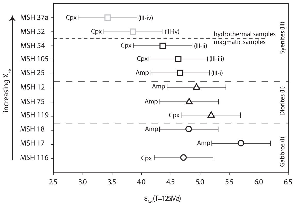
Fig. 11. Age-corrected \epsilon_{Nd} data for representative samples from all units, sorted according to increasing X_{Fe} of the mineral separate analyzed. Clinopyroxene from samples MSH 52 and 37a display hydrothermal textures.
