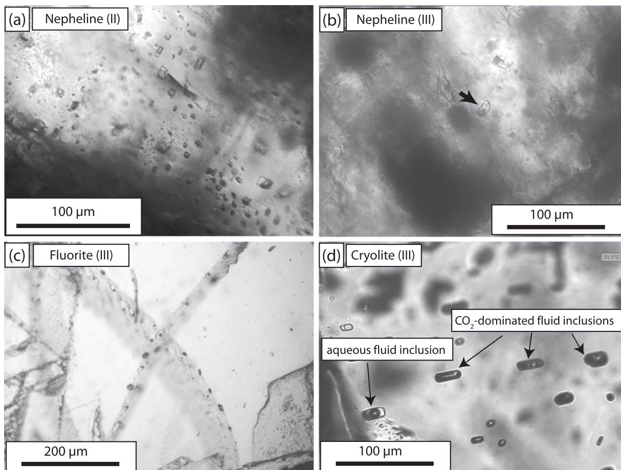
Fig. 15. Photomicrographs of fluid inclusions. (a) Variably sized secondary group (a) CO 2 -rich fluid inclusions in nepheline from diorite; (b) irregularly shaped secondary group (b) aqueous fluid inclusion in nepheline from a syenitic sample; (c) intersecting trails (healed fractures?) of group (b) aqueous fluid inclusions found in a late-stage fluorite in syenites; (d) trail of secondary fluid inclusions consisting of cogenetic CO 2 -dominated [group (a)] and aqueous [group (b)] fluid inclusions in a late-stage cryolite found in a syenite; the identical orientation of carbonic and aqueous fluid inclusions and different volume fractions \phi should be noted.
