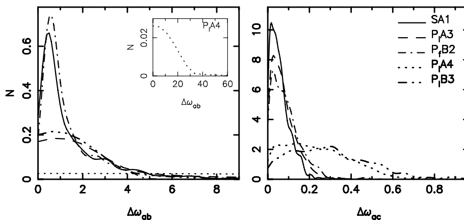
Figure 6. Kernel density distributions of \Delta\omega_{ab} (left-hand panel) and of \Delta\omega_{ac} (right-hand panel) for particles in the haloes SA1, P 1 A3, P 1 A4 and P 1 B3 and as indicated by line legends. Each curve normalized to unit integral. The inset shows the full histogram for P 1 A4 plotted on a different scale.
