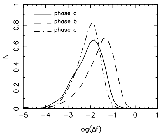
Figure 12. Histograms of frequency drift parameter \log(\Delta f) for the three phases of model SA1 as indicated by the line legends.
