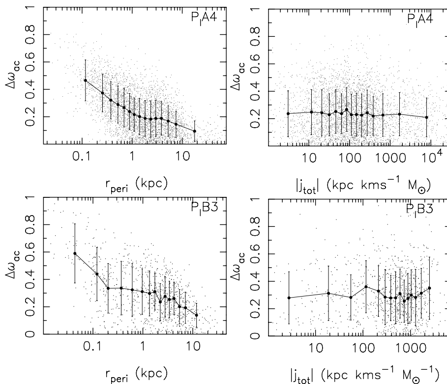
Figure 8. For model P 1 A4 (top panels) and P 1 B3 (bottom panels) left: \Delta\omega_{ac} versus r_{\text{peri}} ; right: \Delta\omega_{ac} versus |j_{\text{tot}}| .
