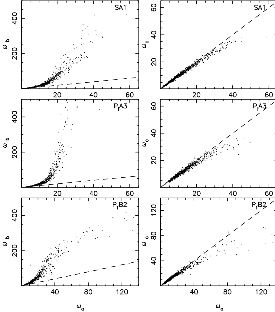
Figure 4. For the three models with extended baryonic components the left-hand panels show \omega_b versus \omega_a and right-hand panels show \omega_c versus \omega_a (frequencies in \text{Gyr}^{-1} ). Dashed lines in each panel show the 1:1 correlation between each pair of frequencies. From top to bottom the models contain a baryonic disc (SA1), a spherical bulge ( P_{fA3} ) and a spherical elliptical ( P_{fB2} ).
