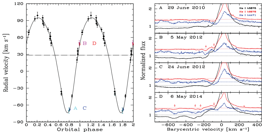
Figure 1. Left-hand panel: orbital radial velocity curve of MWC 314. Two orbital phases B and D when the primary is in front of the secondary ( \phi \sim 0 ), and two quadrature phases A and C ( \phi \sim 0.8 ) are marked. Right-hand panels: the profiles of three He I lines are shown for orbital phases marked A, B, C, and D. DACs are observed in the violet wings of the lines ( marked with arrows ) during the orbital phases B and D. XMM-Newton observed X-rays on 6 May 2014 (D).
