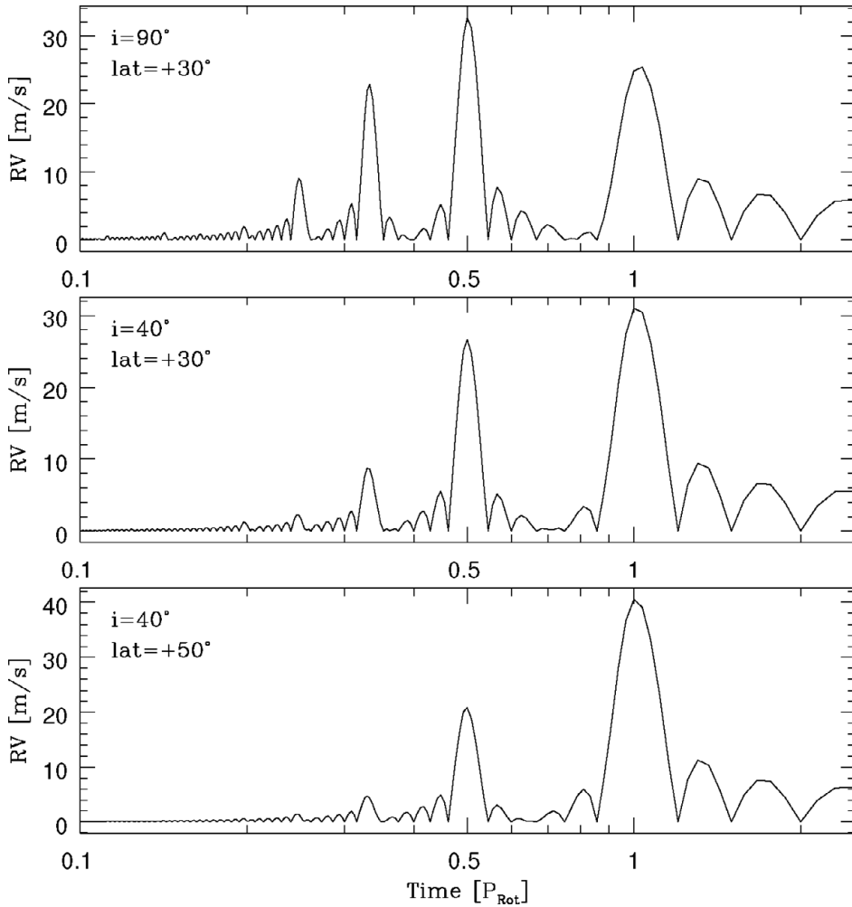
Figure 2. Lomb-Scargle periodograms of the three RV modulations showed in Fig. 1. The fundamental frequency, P_{rot} , and its first harmonics are detected.
