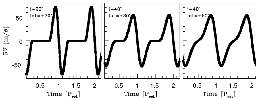
Figure 1. RV modulations due to one spot as a function of time (expressed in rotational period unit). At t=0 , the dark spot of 1% of the visible stellar surface is in front of the line of sight. The shape of the signal changes with the inclination i of the star and the latitude lat of the spot, labelled in the top left of each panel.
