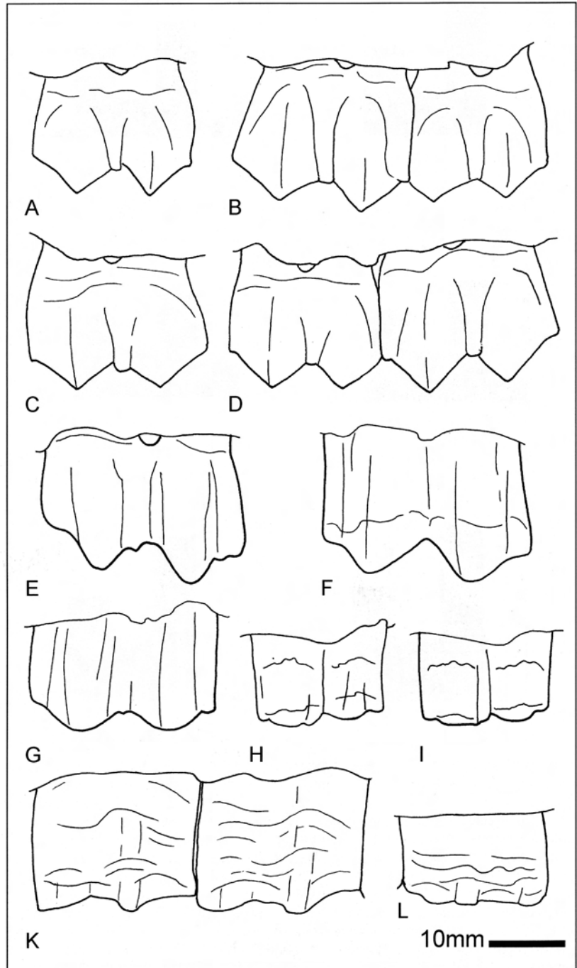
Figure 2. Examples of mesowear. Buccal views of upper molars. A-D: Relief high, Sharp cusps, E-F: Relief high, Round cusps, G: Relief low, Round cusps, H-I: Relief low, Blunt cusps. A) Alces alces left M1, AMNH 2077505; B) Alces alces left M2-M3, AMNH 6408; C) Alces alces right M2, AMNH 19799; D) Alces alces right M2-M3, AMNH 98162; E) Kobus elipsiprymnus right M2, AMNH 53496; F) Alcelaphus buse-laphus right M2, AMNH 31797; G) Alcelaphus buse-laphus right M2, AMNH 216384; H) Damaliscus lunatus right M1, AMNH 82150, I) Damaliscus lunatus right M1, AMNH 82144; K) Equus burchelli left M1-M2, AMNH 82313; L) Equus burchelli right M2, AMNH 27749. AMNH = American Museum of Natural History, New York.
