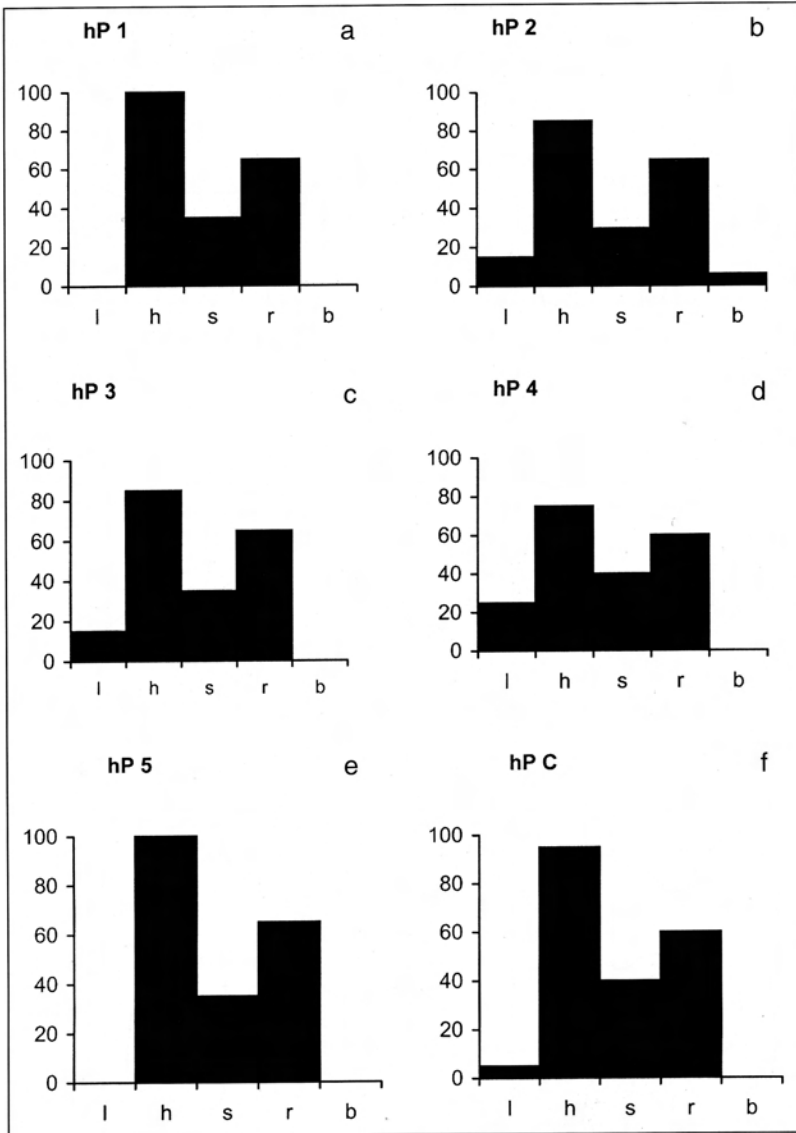
Figure 3. Histograms of mesowear features perlow, perhigh, persharp, perround and perblunt. Histograms are based on the summary values given in Table 2. a-e) experimental data of Hippotherium primigenium ; f) consensus; g) mean; h-k) comparative histograms based on published data by FORTELIUS & SOLOUNIAS (in press); h) hypsodont mixed feeder Aepyceros melampus (impala); i) hypsodont grazer Equus burchelli (Burchell's zebra); k) brachyodont browser Alces alces (moose).
