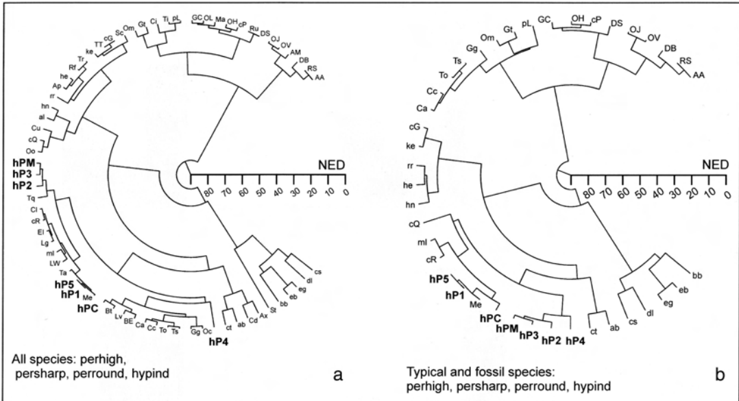
Figure 4. Hierarchical cluster diagrams based on the mesowear features percent high occlusal relief, percent sharp cusps and percent round cusps and the index of hypsodonty from JANIS (1988). a) Clusters based on all recent and fossil species included in this study; b) Clusters based on a set of "typical" recent and fossil species after FORTELIUS & SOLOUNIAS (in press). Symbols as in Table 4, UPPER CASE = BROWSER, lower case = grazer, Mixed case (Capital first) = Mixed-feeder, mixed Case (lower First) = fossil species. Bold = datasets of Hippotherium primigenium . NED = normalized euclidean distance.
