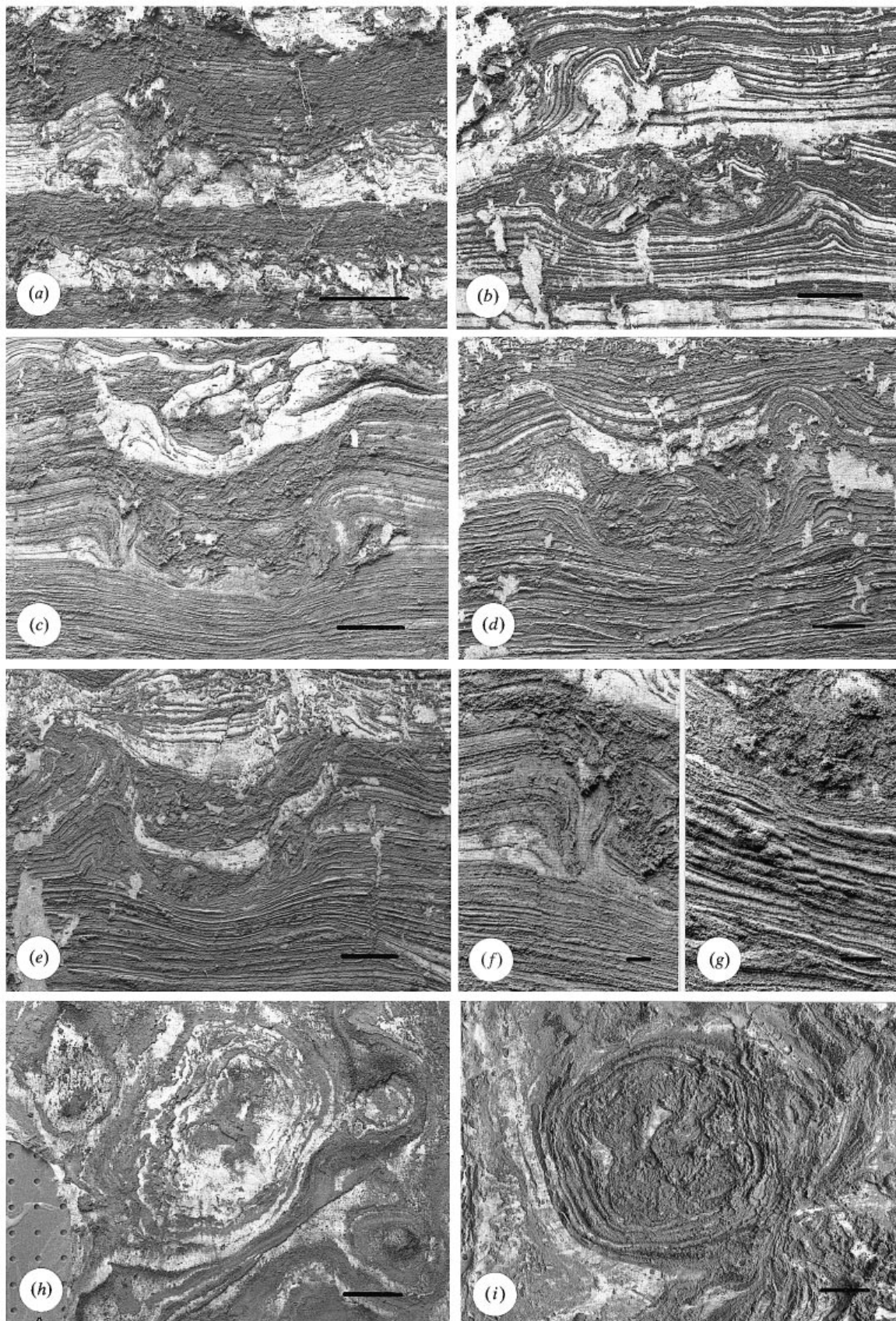
Figure 24. Cattle tracks in the Northwick Formation, Rodley (SO 721123–745107), represented by cellulose acetate peels on muslin (white in photographs). (a–e) Internal-verticle to axial sections showing effects associated with increasing relative penetration. (f) Detail of décollement and layer-thinning in (c). (g) Detail of microfaults beneath footprint in (e). (h, i) Transverse sections through the shaft and overprints. Note in (h) traces of external pits due to dewclaws. Scale bar equivalent to 50 mm in (a–e) and (h, i), and 10 mm in (f, g).
