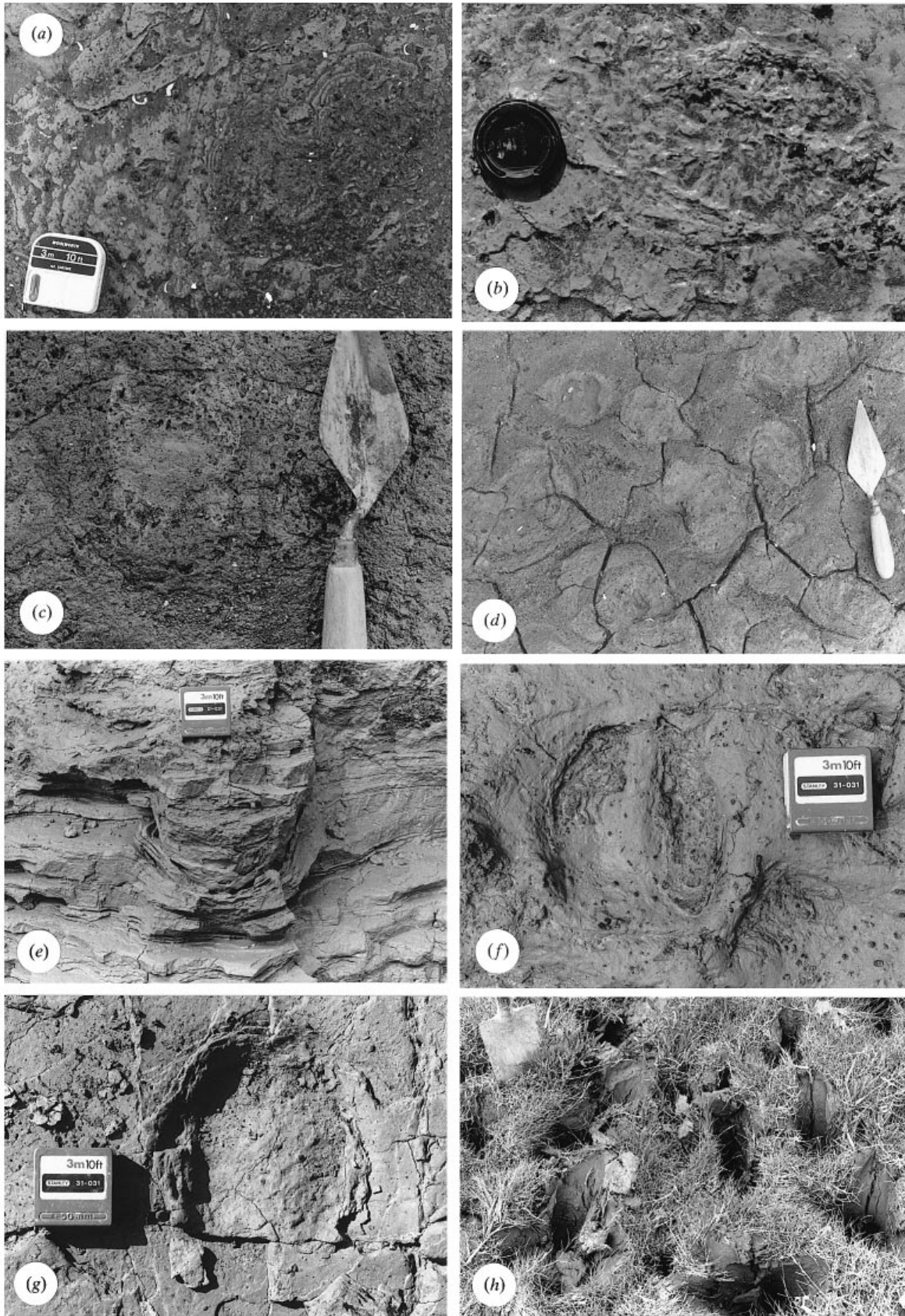
Figure 20. Cattle tracks. (a) lower Wentlooge Formation, Magor Pill (ST 438845). (b) middle Wentlooge Formation, Oldbury Flats (ST 601935). (c) upper Wentlooge Formation, Oldbury Flats (ST 601935). (d) Base of Upper Rumney Formation, Rumney Great Wharf (ST 240779). (e) Deformed zone and shaft-fill, Rumney Formation, Plusterwine (ST 604990). (f) Rumney Formation, Plusterwine (ST 604990). (g) Awre Formation, Frampton-on-Severn (SO 736086). (h) Trampled surface, Northwick Formation, Woolaston (ST 602986). Scales: tape boxes 50 mm square; lens cap 55 mm across; trowel blade 74 mm wide; spade blade 0.135 m wide.
