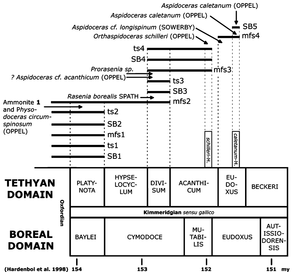
Fig. 16 Possible maximum time ranges of SBs, ts' and mfs' derived from ammonites. Note that SB3, ts3 and SB5 are most precisely dated. The age-assignment of SB1 to ts2 is based on only specimen of Physodoceras circumspinosum (Oppel). The two possible ages given by ammonite 1 (see above) are not considered. Nevertheless, the age assignment given by Lithacosphinctes cf. janus (Choffat) agrees with those given by Physodoceras circumspinosum (Oppel)
