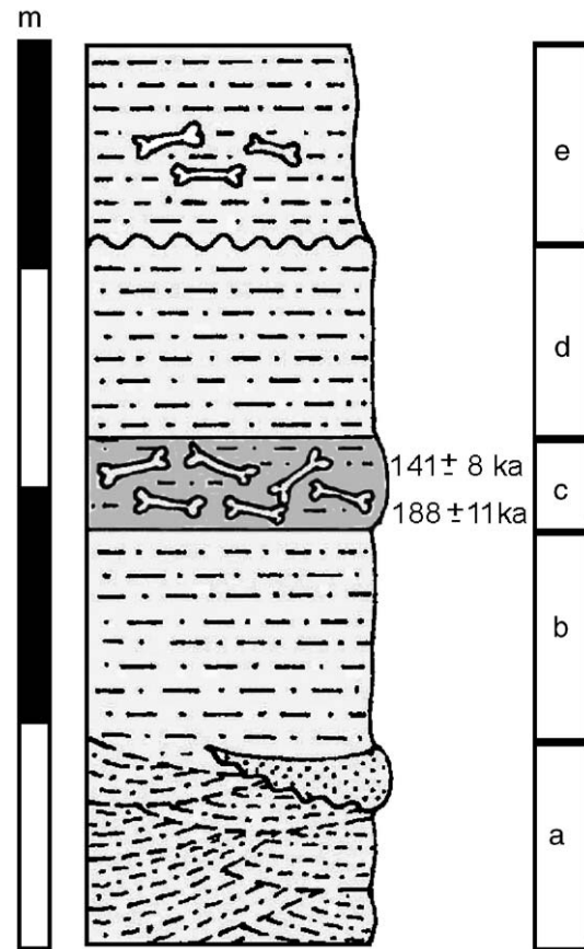
Fig. 2. Stratigraphic column of the La Parte site; (a, b and d) reddish and yellowish sands and silts with black manganese concentrations; (c) lower level (or principal): silts with bones and coprolites accumulations that contain speleothems and calcite. Two samples calcites coming from this level were dated by U-series yielding 188 \pm 11 ka and 141 \pm 8 ka ages; (e) upper level: clays, silts and black organic material with bones.
