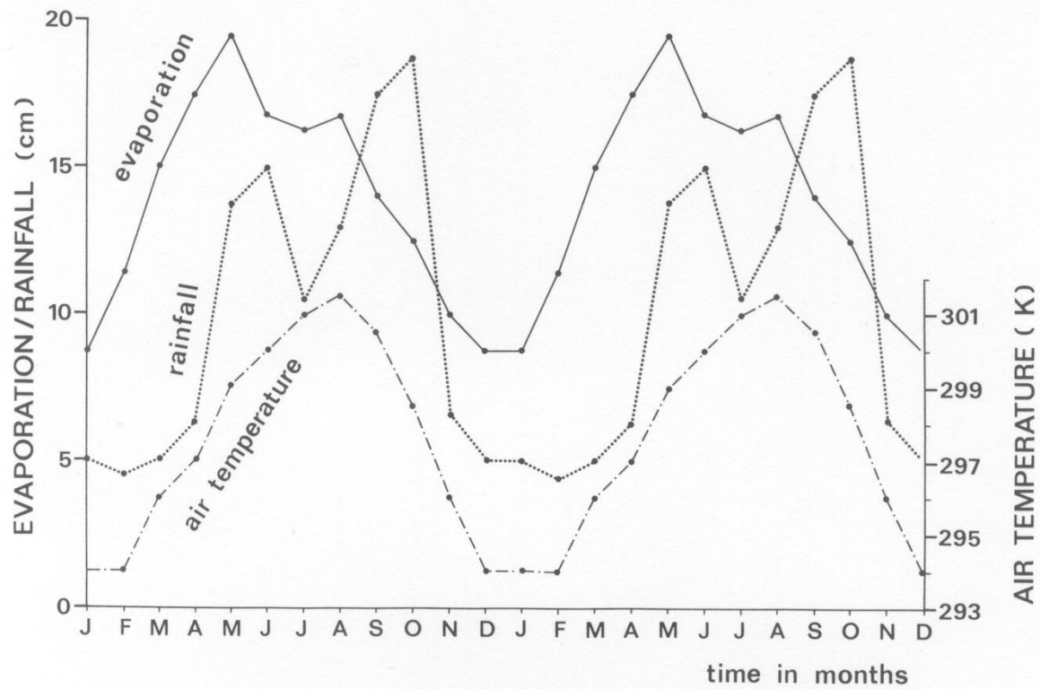
Fig.30 - Seasonal fluctuations in air temperature (-.-), in rainfall (...), and in evaporation (---) in southern Florida (extrapolation of measurements published by Lloyd, 1964).
