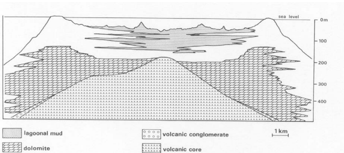
Fig.26 - Distribution of dolomite in the underground of Mururoa Atoll (from Aïssaoui et al., 1986).
