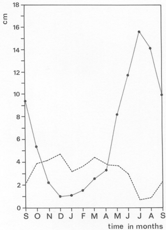
Fig.28 - Seasonal variation in precipitation (---) and evaporation (...) based on averaged meteorological data for the years 1958 to 1973 for the region of Alcázar de San Juan, Spain (from Soriano et al., 1977).
