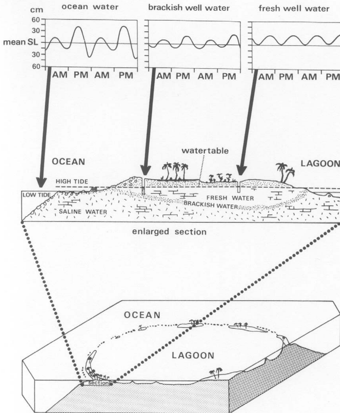
Fig.22 - Tidal periodicity controls the hydrology of atolls: the changes between low- and high water levels are most pronounced at the sea shore, but the brackish water layer and even the fresh water lens (if present) are subject to cyclic variations in its level (from Davis & DeWiest, 1966).
