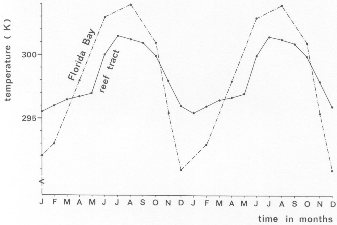
Fig.31 - Seasonal variation in water temperatures in Florida Bay (-.-) and in the Florida reef tract (---) (extrapolation of measurements by Lloyd, 1964).
