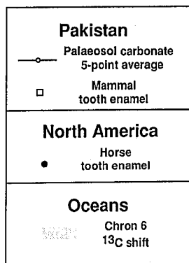
FIG. 1 Isotope transitions in North America and in Pakistan and the late Miocene carbon isotope shift in the oceans. Palaeosols from Pakistan (5-point running average shown as connected circles) 12 , tooth enamel from Pakistan (squares; ref. 16, and our unpublished results) and North America (filled circles). Each shows a 10–12‰ shift between 7 and 5 Myr. The age of the marine carbon shift 30-32 is shown as a dotted area.
