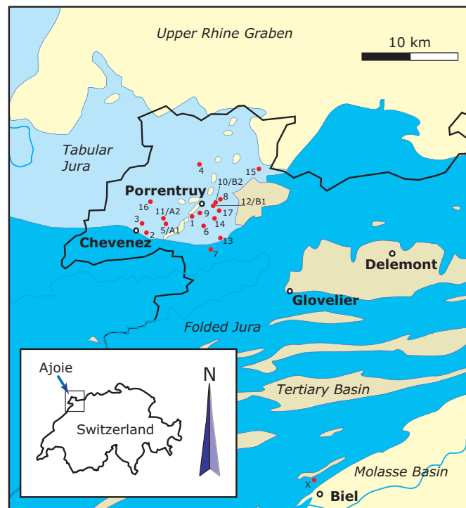
Fig. 1. Geological overview map and Swiss coordinates of locations and geological transects. Note the altitude difference (about 60 m) between the base of Coregent (A1) and the base of the Virgule Marls (A2) in Sur Combed Ronde (note: layers are \pm horizontal; see Swiss geol. map 1085 St-Ursanne).
