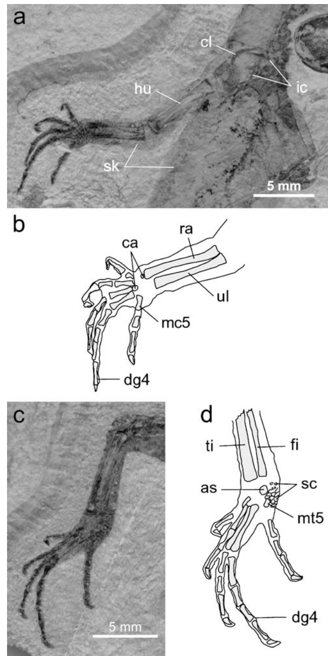
Fig. 3 Daohugou lizard V14386. a The part block, forelimb, and pectoral girdle; b detail of the hand; c the part block, hind limb showing skin traces; d detail of foot showing the enclosure of metatarsals 1–4 in a common skin sheath. as Astragalus, ca carpals, cl clavicle, dg4 digit 4, fi fibula, hu humerus, ic interclavicle, mc5 fifth metacarpal, mt5 fifth metatarsal, ra radius, sc small scales, sk skin traces, ti tibia, ul ulna
