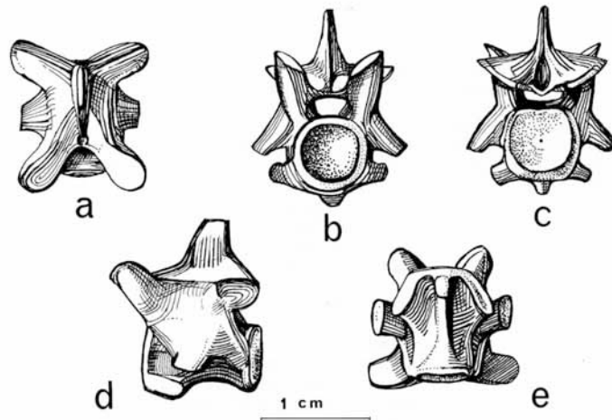
TEXT-FIG. 7. Mesochelys durlstonensis . Cervical vertebra in a , dorsal; b , anterior; c , posterior; d , lateral; e , ventral views.
