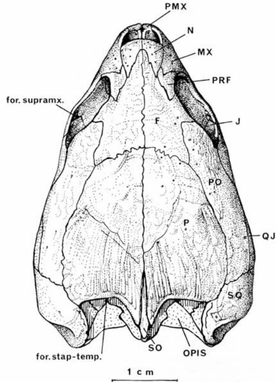
TEXT-FIG. 1. Mesochelys durlstonensis . Skull, slightly restored, in dorsal view.
