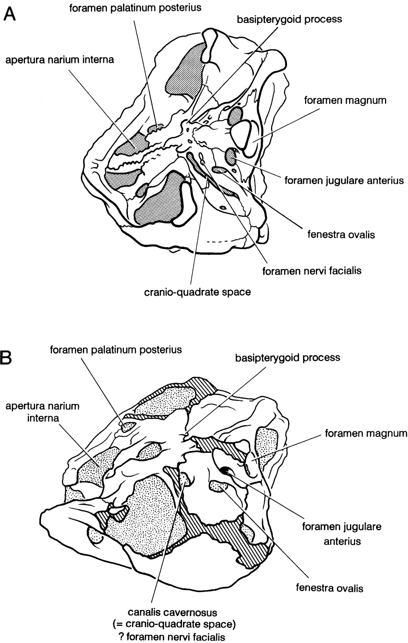
Fig. 23. Comparison of ear regions in posterior oblique views. Anterior is to the left. A. Progonocheilus quenstedti , redrawn from Gaffney, 1990. B. Australocheilus africanus .
