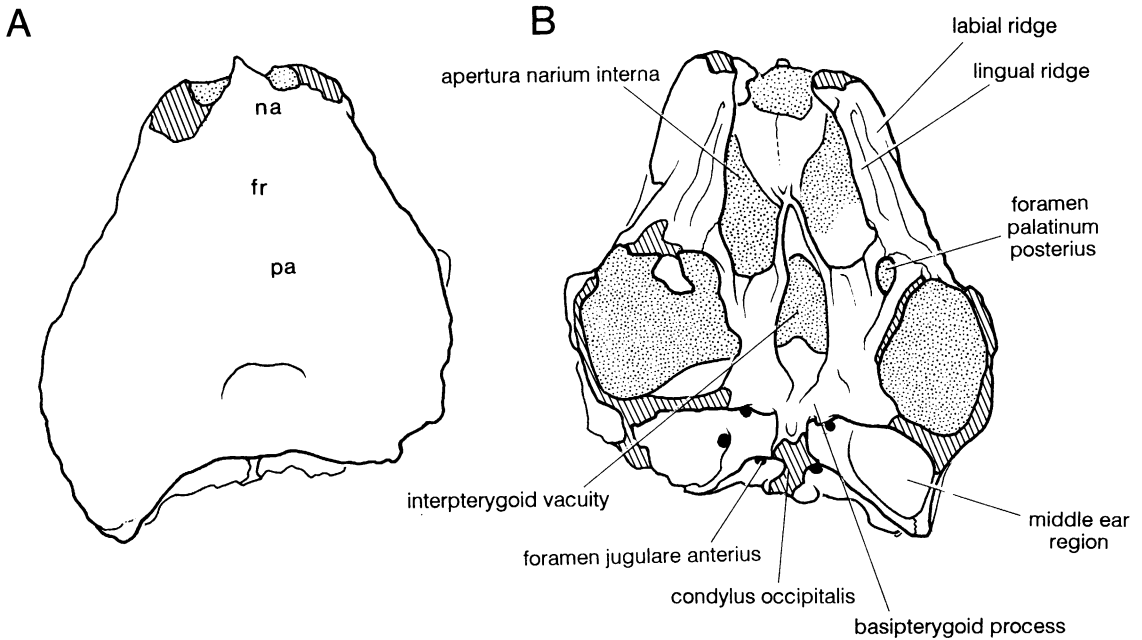
Fig. 3. Australochelys africanus Gaffney and Kitching, 1994, BP/1/4933. A. Dorsal view of skull. B. Ventral view of skull.
