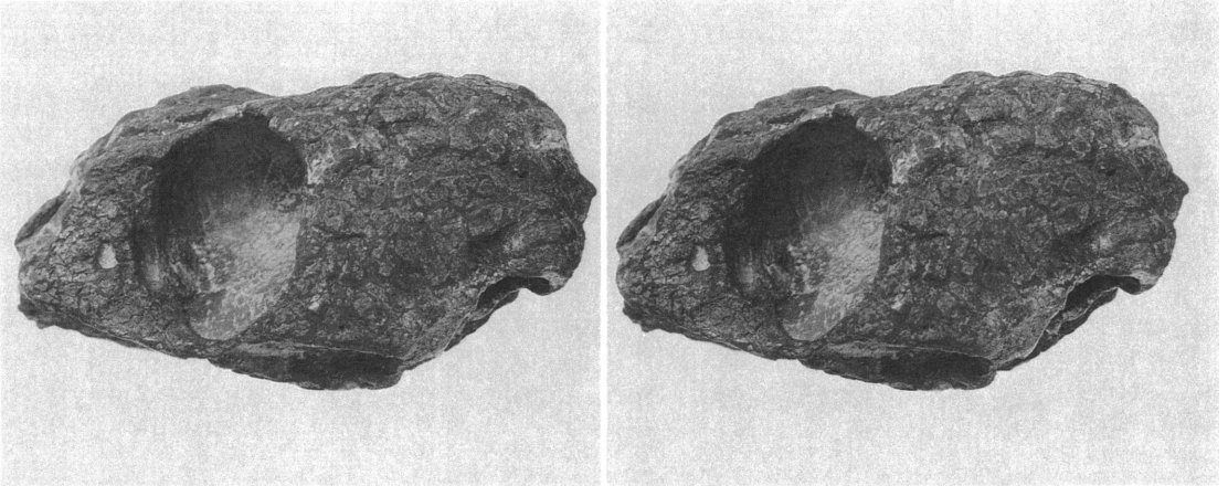
Fig. 4. Australochelys africanus Gaffney and Kitching, 1994, BP/1/4933. Left lateral view of skull. Stereophotograph. See fig. 6A for key.
