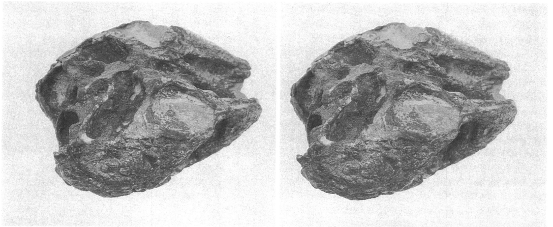
Fig. 13. Australochelys africanus Gaffney and Kitching, 1994, BP/1/4933. Ventrolateral oblique view of left side of skull. Stereophotograph. See fig. 14B for key.
