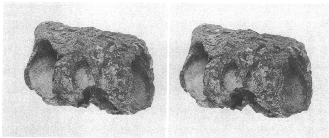
Fig. 8. Australochelys africanus Gaffney and Kitching, 1994, BP/1/4933. Anterior view of skull. Stereophotograph. See fig. 9B for key.
