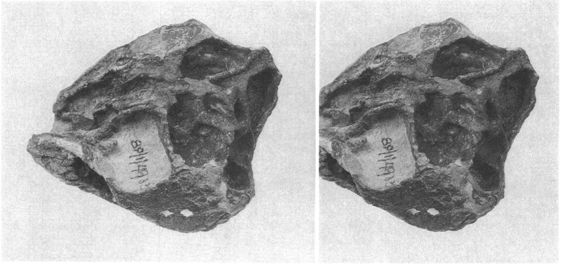
Fig. 12. Australochelys africanus Gaffney and Kitching, 1994, BP/1/4933. Ventrolateral oblique view of right side of skull. Stereophotograph. See fig. 14A for key.
