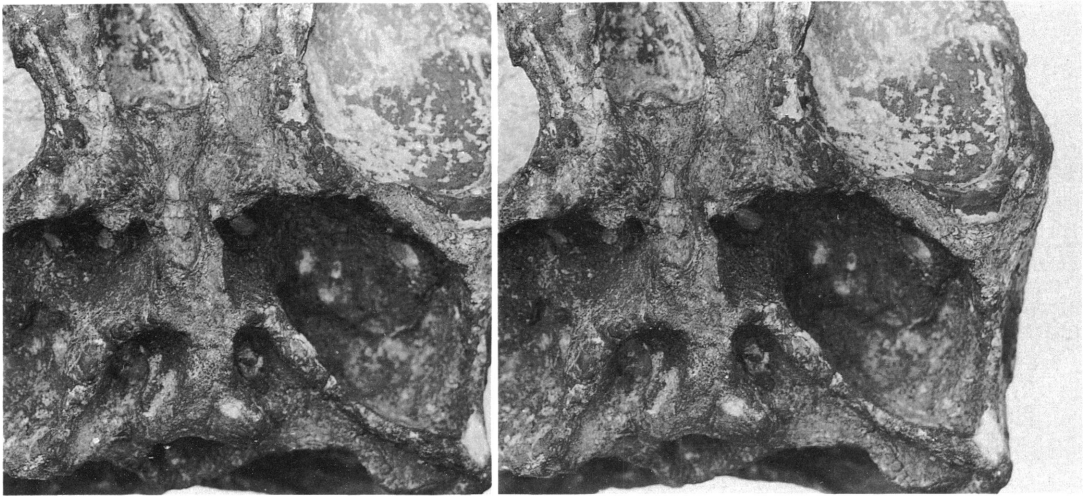
Fig. 15. Australochelys africanus Gaffney and Kitching, 1994, BP/1/4933. Ventral view of left ear region. Stereophotograph. See fig. 16 for key.
