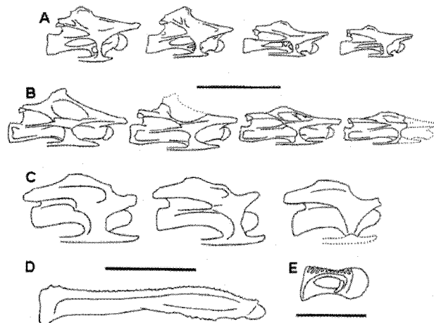
FIGURE 2. Titanosauridae and Brachiosauridae; comparative series illustrating cervical vertebrae in right lateral view. A, Brachiosaurus brancai C5–C8 (HM SI and SII, Janensch, 1950). B, Sauroposeidon proteles C5–C8 (OMNH 53062). C, unnamed titanosaurid C4, C7, and C8 (DGM serie a, Powell, 1987). D, Unnamed taxon (YPM 5294; Ostrom, 1970). E, Pleurocoelus nanus (USNM 5678, Marsh, 1888). Scale bars equal 1 m, A, B; 20 cm, C, D; 10 cm, E.
