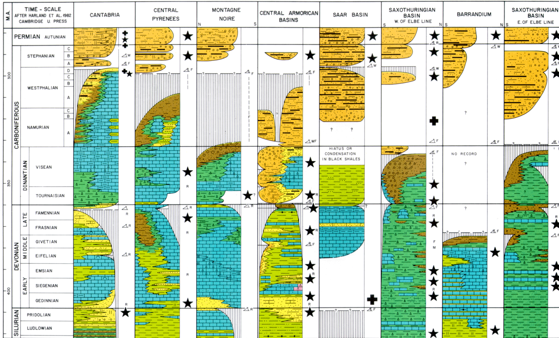
PALAEZOIC, BASINS LOCATED WITHIN VARISCAN FOLD BELT
