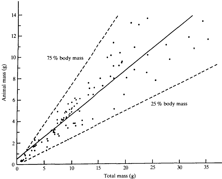
Fig. 2. Hermit crab mass without snail shell compared to the total mass (crab plus shell). Each point represents a single animal. The solid line is the least-squares regression line. The dashed lines indicate where the crab is 25 % and 75 % of the total mass.
