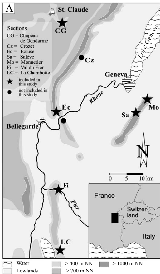
Fig. 6. (A) Study area. (B) Study interval (shaded). Be3–Va3 are major ‘third-order’ SBs identified by Hardenbol et al. (1998). Well-expressed discontinuity surfaces and zones of surfaces corresponding to SBs, TS, and sequence-boundary zones (SBZ) observed in the study area correlate well with the ‘global’ sequence-stratigraphic scheme (data from; Le Hégarat, 1971, 1980; Remane, 1985; Gradstein et al., 1995; Hardenbol et al., 1998; Hillgärtner, 1999; Clavel et al., 1986).
