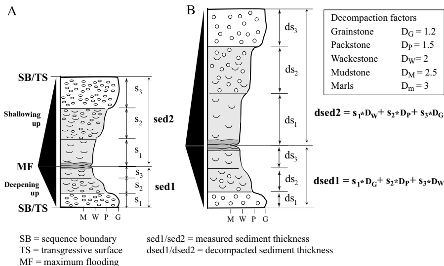
Fig. 1. Decompaction of a small-scale depositional sequence representing one cycle of relative sea-level change. (A) Measured thickness of different sediment textures (s 1 –s 3 ) in lowstand/transgressive deposits (sed1) and highstand deposits (sed2) of a depositional sequence. (B) Decompacted thickness (dsed1/dsed2) calculated with indicated decompaction factors.
