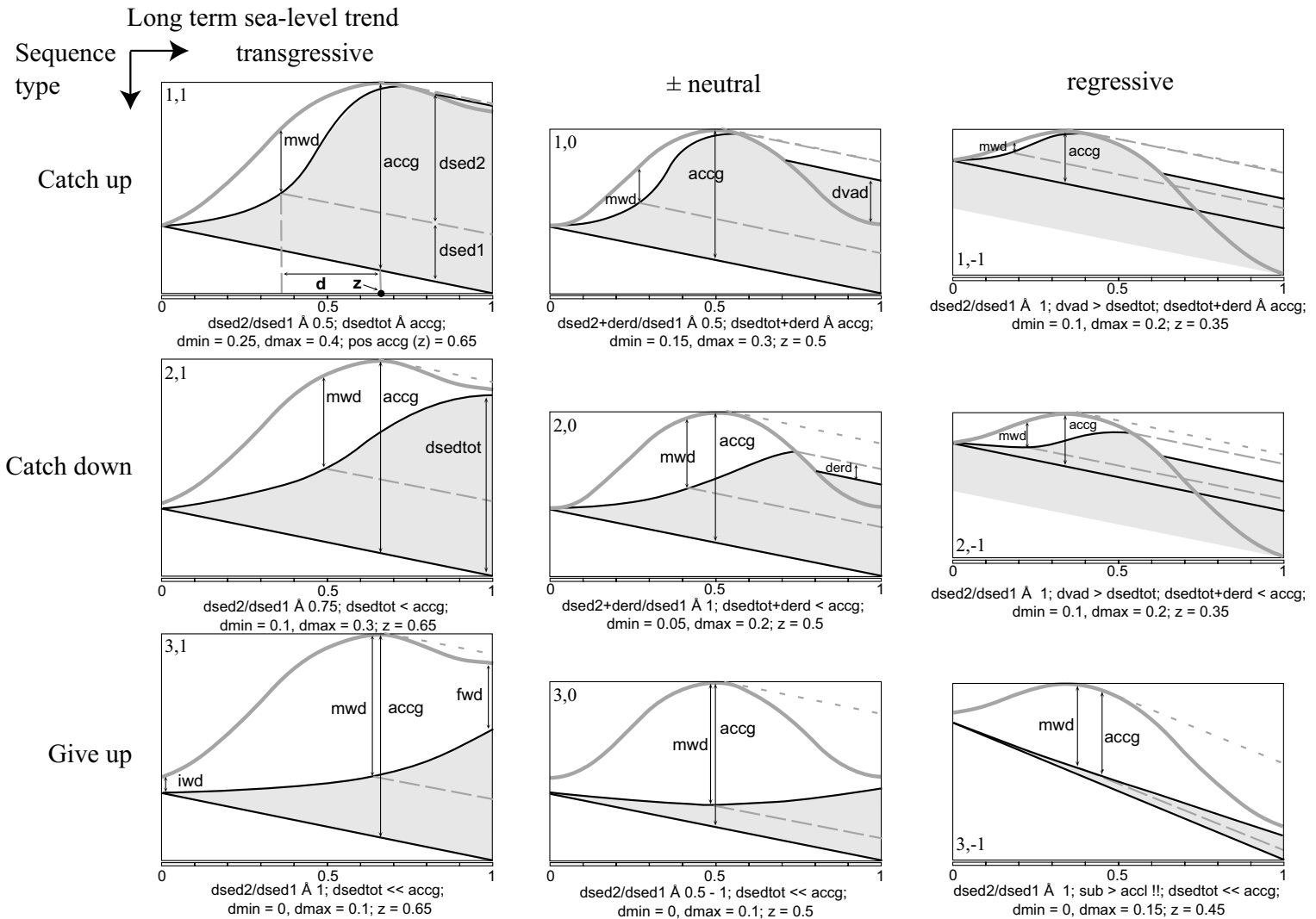
Fig. 5. Nine combinations of three sequence types with different trends in long-term sea level. For each combination minimum and maximum values for d and the position of the maximum accg(z) are estimated in relative time units.
