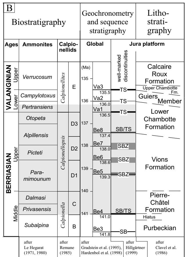
Fig. 6. (A) Study area. (B) Study interval (shaded). Be3–Va3 are major ‘third-order’ SBs identified by Hardenbol et al. (1998). Well-expressed discontinuity surfaces and zones of surfaces corresponding to SBs, TS, and sequence-boundary zones (SBZ) observed in the study area correlate well with the ‘global’ sequence-stratigraphic scheme (data from; Le Hégarat, 1971, 1980; Remane, 1985; Gradstein et al., 1995; Hardenbol et al., 1998; Hillgärtner, 1999; Clavel et al., 1986).
