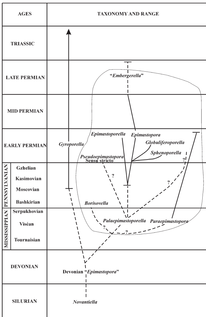
Fig. 2. Composition and stratigraphic range of the Epimastoporellinae n. subtrib. compared with some other Gyroporelleae.
