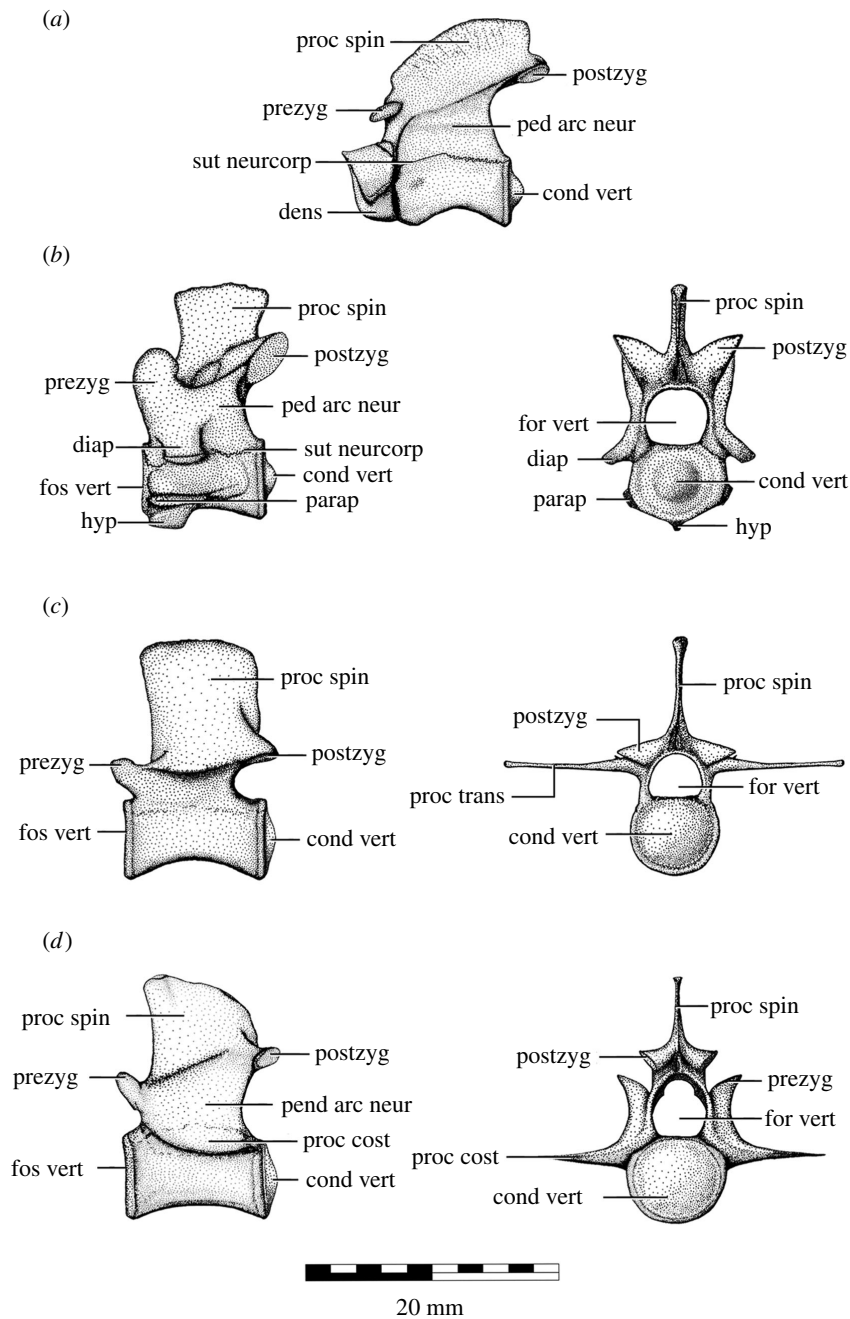
Figure 3. Axial osteology of Isisfordia duncani gen. et sp. nov. Schematic interpretations of selected vertebrae from QM F36211 (holotype): (a) axis in left lateral aspect; (b) cervical vertebra III in left lateral and caudal aspect; (c) lumbar vertebra III(?) in left lateral and caudal aspect; (d) caudal vertebra I in left lateral and caudal aspect. Abbreviations: cond vert, vertebral condyle; dens, dens; diap, diapophysis; for vert, vertebral foramen; fos vert, vertebral fossa; hyp, hypopophysis; parap, parapophysis; ped arc neur, peduncle of the neural arch; postzyg, postzygopophysis; prezyg, prezygopophysis; proc cost, costal process; proc spin, spinal process; proc trans, transverse process; sut neurcorp, neurocorpal suture.
