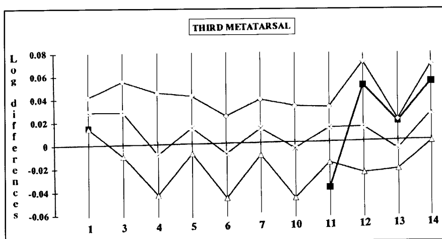
FIG. 5. Logarithmic ratio diagram comparing the third metatarsal of the Taghar Hipparion with H. molayanense . Standard = H. mediterraneum , Pikermi, n = 11-64 (Koufos, 1987a); ■ = H. sp. cf. H. molayanense , Taghar, n = 1-2; x = H. molayanense , Molayan, mean values, n = 8-12; Δ = H. molayanense , min values; ◇ = H. molayanense , max values (Zouhri, 1992a).
