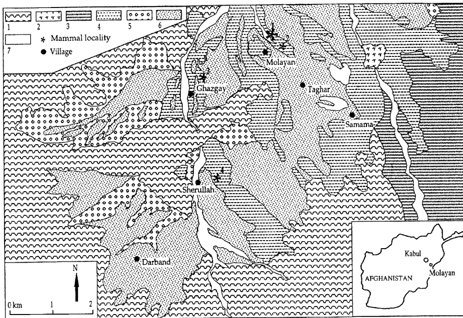
FIG. 1. Geological map of the southern part of the Khurdkabul Basin (after Mennessier, 1974, modified) and the location of some mammal localities. 1) Molayan, 2) Taghar, 3) Ghazgay and 4) Sherullah. Lithologic legend : 1) Metamorphic rocks of the « Série de Kaboul » ; 2) Diorites ; 3) Cretaceous schists of the « Série de Kotagae » ; 4) Neogene deposits of the « Série de Lataband » ; 5) old terraces and screes ; 6) new terraces and screes ; 7) recent alluvium.
