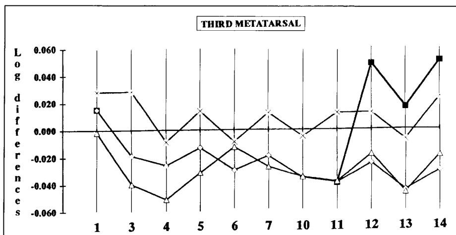
FIG. 4. Lorgarithmic ratio diagram comparing the third metatarsal of the Taghar Hipparion with other species. Standard = H. mediterraneum , Pikermi, n = 11-64 (Koufos, 1987a); ■ = H. sp. cf. H. molayanense , Taghar, n = 1-2; x = H. molayanense , Molayan, mean values, n = 8-12 (Zouhri, 1992a); ◊ = H. dietrichi , « Prochoma I », Macedonia, Greece (Koufos, 1987b); Δ = H. dietrichi , Vathyakkos, Macedonia, Greece (Koufos, 1988).
