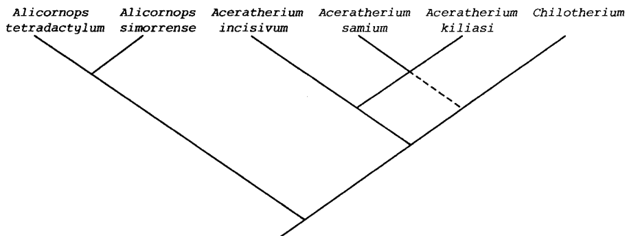
Text-fig. 9. Hypothesis of phylogenetic relationships among the upper miocene eurasiatic Aceratherium .
