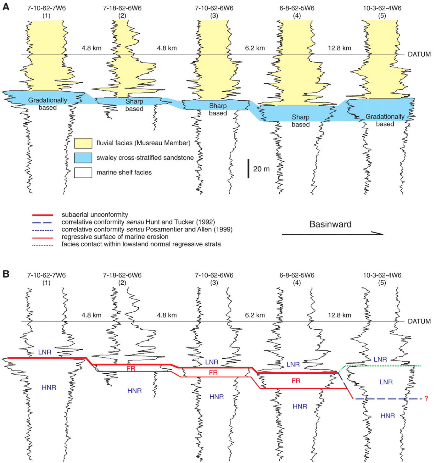
Fig. 29. Sequence stratigraphic interpretation of the swaley cross-stratified sandstone of the Kakwa Member (Cardium Formation), and adjacent units (modified after Plint, 1988 ). A. Sedimentary facies. As constrained by outcrop and core studies, the contact between the fluvial and the underlying shoreface facies is unconformable in wells (1), (2), (3) and (4), and conformable in well (5). B. Sequence stratigraphic interpretation. Correlative conformities are difficult to detect on well logs, within regressive successions of coarsening-upward shallow-marine facies. Correlative conformities are easier to detect on seismic lines, where stacking patterns such as offlap can be observed (e.g., Fig. 7 ). Note the downstepping of the subaerial unconformity during forced regression; the thinning of sharp-based shoreface deposits toward the basin margin; and the aggradation recorded by the lowstand normal regressive strata. In this example, gradationally-based shoreface deposits indicate normal regression (highstand to the left; lowstand to the right), whereas sharp-based shoreface deposits are diagnostic for forced regression. This criterion allows the separation between normal and forced regressive deposits even in the absence of seismic data. Abbreviations: FR – forced regressive; HNR – highstand normal regressive; LNR – lowstand normal regressive.
