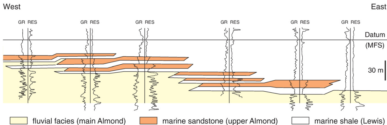
Fig. 20. Regional well-log cross-section of the Almond Formation in the Washakie Basin, Wyoming (modified from Weimer, 1966; Martinsen and Christensen, 1992; and C. Bartberger, pers. comm.) The backstepping stacking pattern of parasequences records the westward transgression of the Western Interior Campanian Seaway. The cross-section is approximately 65 km long. Well logs shown: gamma ray (GR) and resistivity (RES).
