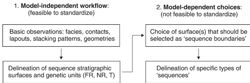
Fig. 22. The method of sequence stratigraphy: standardized workflow versus model-dependent choices. The model-independent workflow leads to the subdivision of the stratigraphic section into a succession of genetic units (systems tracts) separated by sequence stratigraphic surfaces. Once this sequence stratigraphic framework is built, the interpreter may make model-dependent choices with respect to the selection of surfaces that should be elevated to the status of sequence boundary. The nomenclature of sequence stratigraphic surfaces and systems tracts is also model-dependent to some extent (Fig. 10), but a standard set of terms can be recommended to facilitate communication between all practising geoscientists. The nomenclature of systems tracts is particularly difficult to reconcile (Fig. 4), which is why the definition of genetic units with reference to shoreline trajectories (i.e., forced regressive; lowstand and highstand normal regressive; transgressive) offers an unbiased solution to this problem. Abbreviations: FR – forced regressive; NR – normal regressive (lowstand and highstand); T – transgressive.
