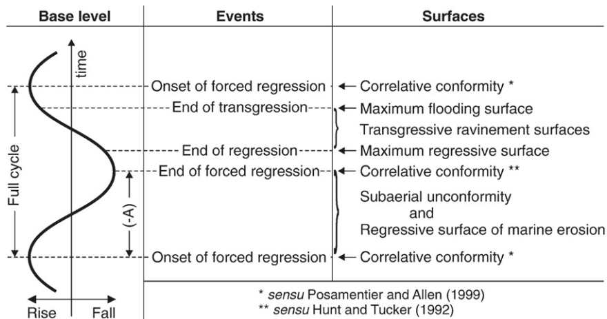
Fig. 15. Timing of the seven surfaces of sequence stratigraphy relative to the four events of the base-level cycle (from Catuneanu, 2006). The reference curve of base-level change reflects fluctuations in base level along the coastline. The timing of the four events is unique along each dip line, but it may change along strike due to variations in sediment supply and/or subsidence rates. Although a symmetrical reference curve is used here (and in Fig. 16) for illustrative purposes, the actual curve may be either symmetrical or asymmetrical, depending on the interplay between the various driving mechanism(s) responsible for the fluctuations in base level. The erosion that generates transgressive ravinement surfaces may be triggered by waves or tides (hence the usage of plural). Abbreviation: (-A) – negative accommodation.
