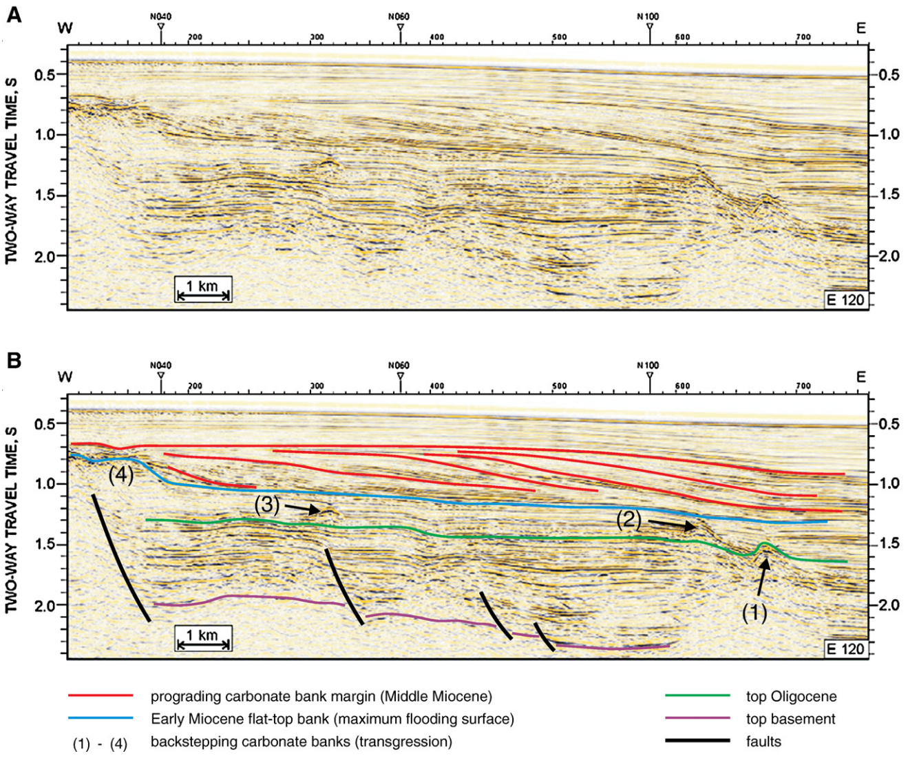
Fig. 21. Uninterpreted (A) and interpreted (B) seismic line showing updip and downdip shifts of a carbonate bank margin (Oligocene–Miocene, Maldives Islands, Indian Ocean; modified from Belopolsky and Droxler, 2003). Depositional trends change from retrogradation (transgression: late Oligocene to early Miocene) to progradation (highstand normal regression: middle Miocene). On seismic lines, the pattern of backstepping is often easier to observe in carbonates than it is in siliciclastics (compare with Fig. 19). The boundary between the transgressive and highstand systems tracts is represented by the maximum flooding surface (downlap surface).
