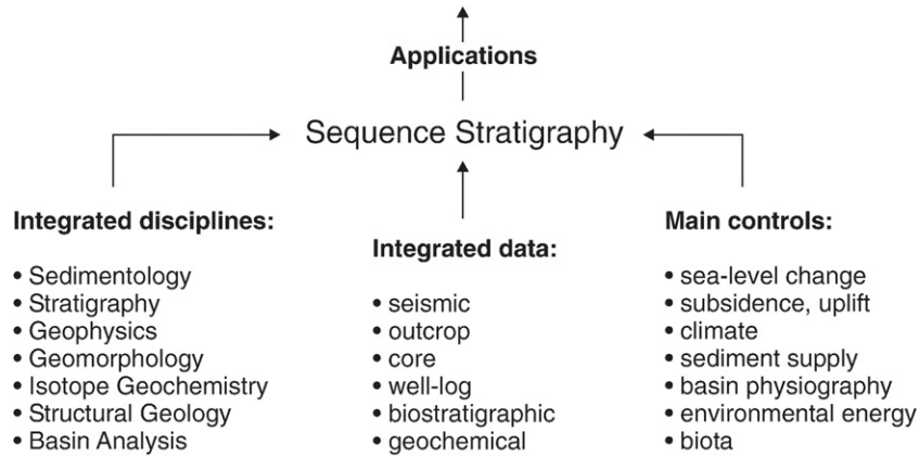
Fig. 1. Sequence stratigraphy in the context of interdisciplinary research.
