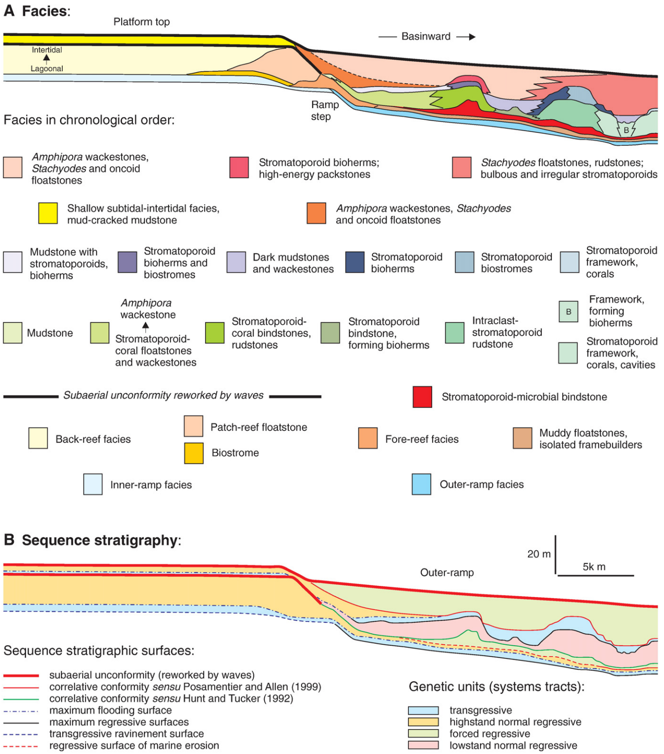
Fig. 32. Architecture of facies, genetic units (systems tracts) and sequence stratigraphic surfaces of a Late Devonian reef system that developed on a gently sloping, epicontinental ramp (Alexandra Formation, Western Canada Sedimentary Basin; modified from MacNeil and Jones, 2006). Vertical exaggeration is 250 times.
