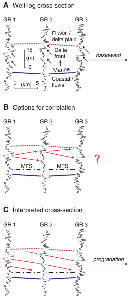
Fig. 9. Workflow in the correlation of well logs in a transitional marine to nonmarine setting (Upper Cretaceous, central Alberta). A. Well-log cross-section: arrows indicate coarsening-upward trends, interpreted as prograding lobes (or 'parasequences'), on the gamma-ray (GR) logs. The solid line of correlation is a transgressive wave-ravinement surface (base of transgressive marine deposits). The dotted correlation line is a facies contact at the top of delta front facies. B. Options for the correlation of the prograding lobes. The selection of the option that makes most geological sense is based on a facies model of deltaic progradation which indicates that clinoforms downlap the maximum flooding surface in a basinward (i.e., easterly) direction (C). The maximum flooding surface (MFS) is interpreted at the top of the fining-upward trends that overlie the transgressive wave-ravinement surface. C. Interpreted cross-section: the steps involved in the interpretation include (1) the identification of prograding lobes on individual well logs (A), and (2) the correlation of these lobes between isolated data control points (well logs in this case) based on the predictions of a facies model of deltaic progradation (C).
