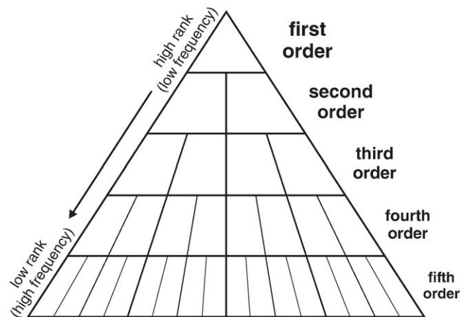
Fig. 26. Diagrammatic representation of the concept of hierarchy. The use of hierarchical orders ('low' versus 'high') in the literature is inconsistent: some refer to first-order cycles as 'high order', making reference to the high position within the hierarchy pyramid, whereas others refer to first-order cycles as 'low order', making reference to the numbering system (1 is lower than 2, etc.). For this reason, we use the less ambiguous terms of 'high rank' versus 'low rank'. These terms make reference to the position of the cycle within the hierarchy pyramid.
