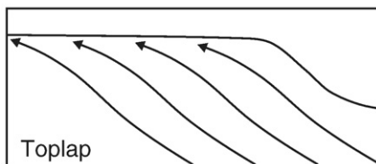
Fig. 13. Stratal terminations that can be observed above or below a stratigraphic surface in seismic profiles and larger scale outcrops (from Mitchum and Vail, 1977).
