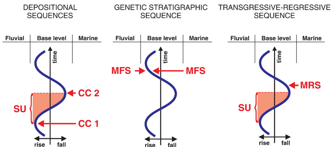
Fig. 24. Selection of sequence boundaries according to the 'depositional', 'genetic stratigraphic' and 'transgressive-regressive' sequence models. The choice of sequence boundary is less important than the correct identification of all sequence stratigraphic surfaces in a succession (Fig. 10). Abbreviations: SU – subaerial unconformity; CC 1 – correlative conformity sensu Posamentier and Allen (1999); CC 2 – correlative conformity sensu Hunt and Tucker (1992); MFS – maximum flooding surface; MRS – maximum regressive surface. The subaerial unconformity is a stage-significant surface, whereas all other surfaces shown in this diagram are event-significant (Figs. 15, 16).
