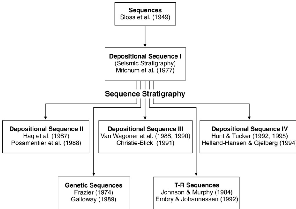
Fig. 3. Sequence stratigraphic models (from Catuneanu, 2006; modified after Donovan, 2001).
