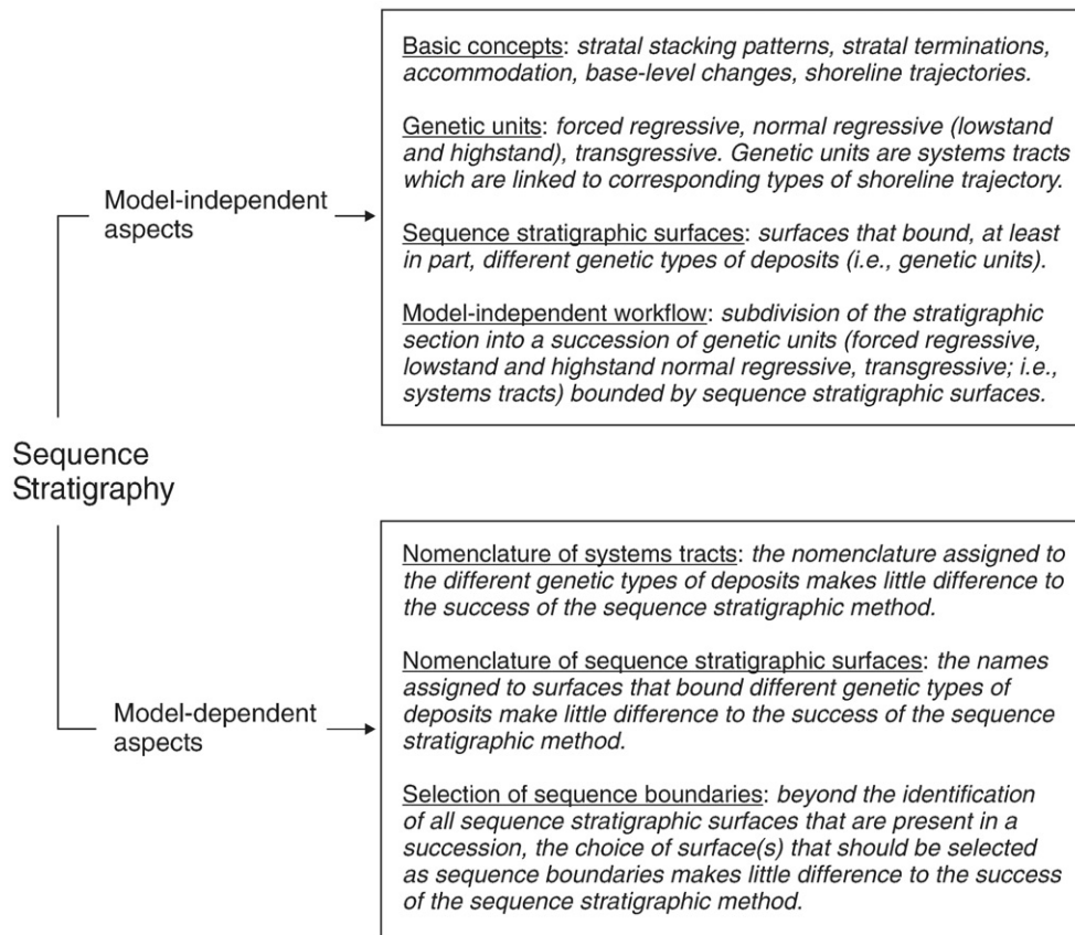
Fig. 10. Model-independent versus model-dependent aspects of sequence stratigraphy. The model-independent aspects form the core platform of the method that is validated by all 'schools'. The model-dependent aspects can be left to the discretion of the practitioner; such flexibility allows one to adapt more easily to the particularities of each case study. Depending on situation, any one of the models may provide the optimum approach to the sequence stratigraphic analysis. For example, the selection of sequence boundaries may depend on depositional setting or the type of data available for analysis.
