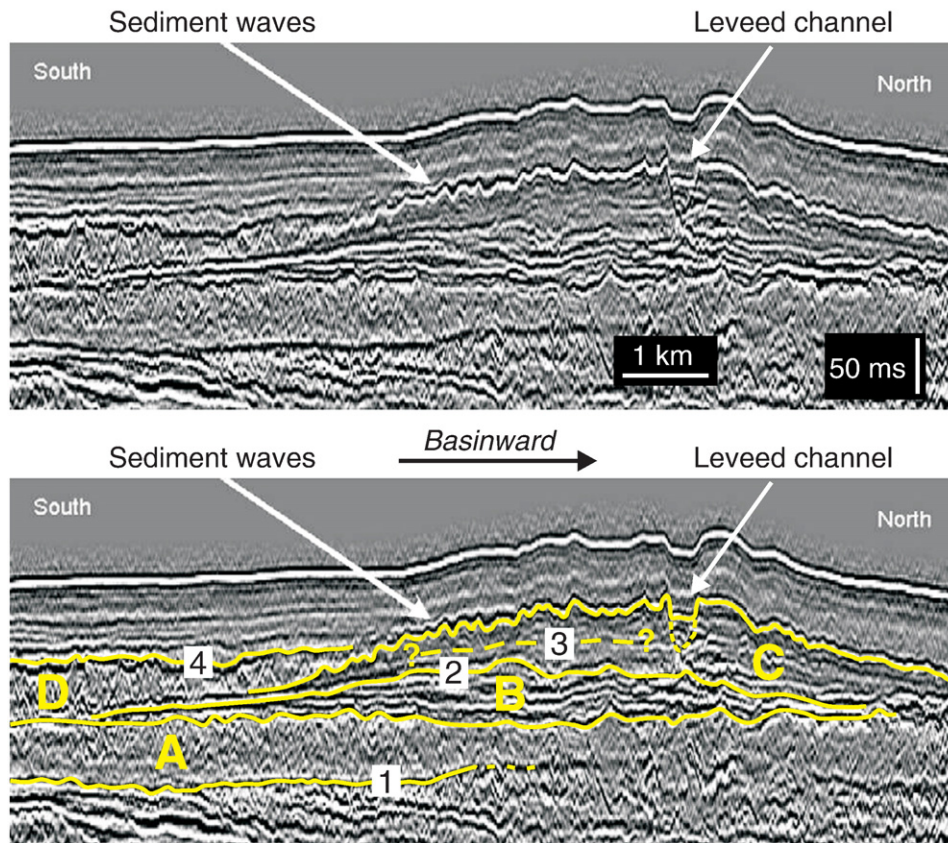
Fig. 31. Uninterpreted and interpreted seismic lines showing a complete basin-floor succession of gravity-flow deposits formed in response to a full cycle of base-level changes (modified from Posamentier and Kolla, 2003). A – mudflow deposits (chaotic internal facies): early stage of forced regression; B – turbidity-flow frontal splay (well-defined parallel reflections): late stage of forced regression; C – leveed channel and overbank facies (high-amplitude reflections associated with the sandy channel fill and weak reflections/transparent facies associated with the finer grained overbank deposits): lowstand normal regressive and early transgressive deposits; D – mudflow deposits (chaotic internal facies): late transgressive deposits. Note the gradual progradation of gravity-flow deposits into the basin from A to C, and the retrogradation from C to D. Sequence stratigraphic surfaces: 1 – correlative conformity sensu Posamentier and Allen (1999); 2 – correlative conformity sensu Hunt and Tucker (1992); 3 – maximum regressive surface (cryptic, within an undifferentiated succession of low-density leveed-channel turbidites); and 4 – maximum flooding surface.
