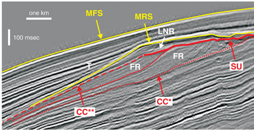
Fig. 7. Seismic line in the Gulf of Mexico showing different genetic types of deposits (forced regressive, normal regressive, transgressive) and stratigraphic surfaces that may serve as sequence boundaries according to different sequence stratigraphic models (modified from Posamentier and Kolla, 2003). Abbreviations: FR – forced regressive; LNR – lowstand normal regressive; T – transgressive; SU – subaerial unconformity; CC* – correlative conformity sensu Posamentier and Allen, 1999 (=basal surface of forced regression); CC** – correlative conformity sensu Hunt and Tucker, 1992; MRS – maximum regressive surface; MFS – maximum flooding surface. The line displays the typical stacking patterns and stratal terminations associated with forced regression (offlap, downlap, toplap, truncation), normal regression (downlap, topset), and transgression (onlap).
