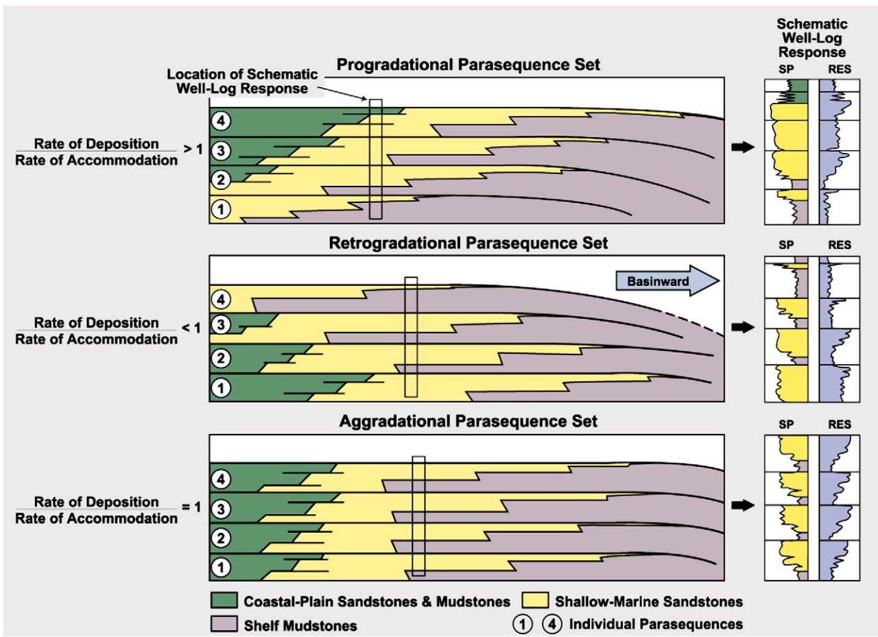
Fig. 12. Vertical stacking of parasequence sets (from Van Wagoner et al., 1990).
