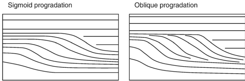
Fig. 14. Stratal geometries associated with a prograding shelf-slope system (from Mitchum and Vail, 1977). A sigmoid geometry indicates positive accommodation on the shelf during progradation. An oblique geometry indicates little or no accommodation on the shelf during progradation.
