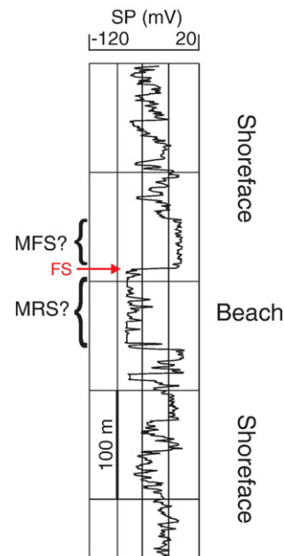
Fig. 8. Spontaneous potential (SP) log from a dominantly shallow-water succession in the Gulf of Mexico. The log illustrates the uncertainty that can affect the placement of the maximum regressive and maximum flooding surfaces in the case of monotonous lithological successions that lack obvious grading trends. The same problem affects the interpretation of outcrops which expose ‘massive’ beds (no grading). In this example, the uncertainty is in the range of tens of meters. Abbreviations: FS – flooding surface; MRS – maximum regressive surface; MFS – maximum flooding surface.
