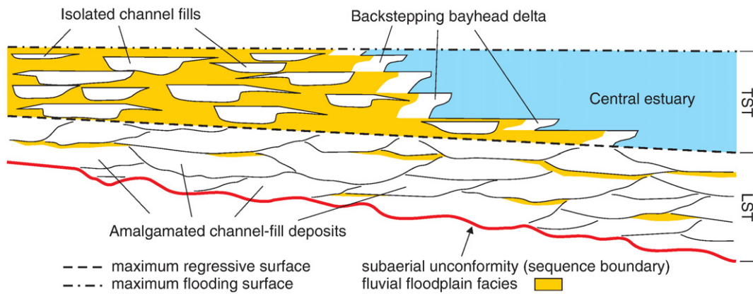
Fig. 27. Dip-oriented stratigraphic cross-section through fluvial to estuarine deposits (modified after Kerr et al., 1999). The lowstand systems tract (LST – lowstand normal regressive deposits) is composed of amalgamated channel-fill facies (low-accommodation conditions) resting on a subaerial unconformity with substantial erosional relief. The transgressive systems tract (TST) consists of floodplain-dominated facies (isolated ribbons encased within floodplain facies, deposited under high-accommodation conditions) and correlative estuarine facies towards the coastline. The maximum regressive surface may be traced at the base of the oldest central estuary facies, and at the contact between amalgamated channel fills and the overlying floodplain-dominated facies farther inland. In this case study, fluvial processes are dominated by ‘downstream controls’ (marine base-level changes). Farther upstream, the maximum regressive surface may eventually onlap the subaerial unconformity.
