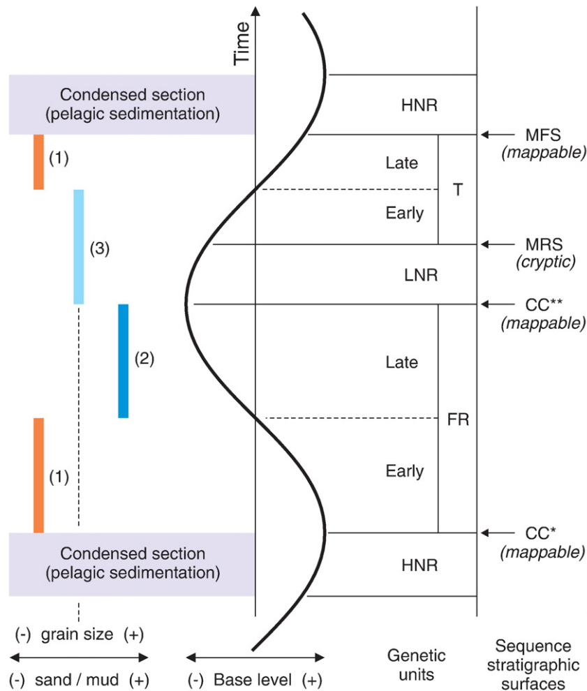
Fig. 30. Dominant types of gravity-flow deposits that form the submarine fan complex in a deep-water setting (modified from Posamentier and Kolla, 2003; Catuneanu, 2006): (1) mudflow deposits, dominated by lobes; (2) high-density turbidites, dominated by frontal splays; (3) low-density turbidites, dominated by leveed channels. The sequence stratigraphic interpretation of the submarine fan complex is more challenging where correlation with the coastal and shallow-water settings cannot be established. However, the predictable change in sediment supply to the deep-water setting during the various stages of the base-level cycle allows for the construction of a sequence stratigraphic framework. See text for more details. Abbreviations: HNR – highstand normal regressive deposits; FR – forced regressive deposits; LNR – lowstand normal regressive deposits; T – transgressive deposits; CC* – correlative conformity sensu Posamentier and Allen (1999); CC** – correlative conformity sensu Hunt and Tucker (1992); MRS – maximum regressive surface; MFS – maximum flooding surface. See Fig. 31 for a case study.
