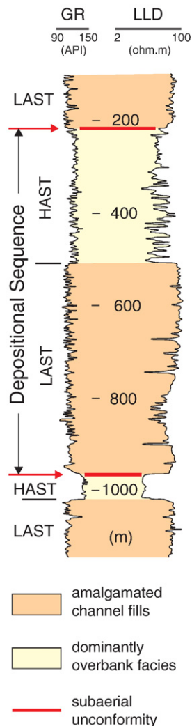
Fig. 28. Fully fluvial succession in an overfilled foreland basin (Miocene, Assam Basin, India; well logs courtesy of the Oil and Natural Gas Corporation, India). The fluvial succession consists of depositional sequences bounded by subaerial unconformities. Abbreviations: LAST – low-accommodation systems tract; HAST – high-accommodation systems tract. The preserved thicknesses of the low- and high-accommodation systems tracts depend on: (1) the spans of time when the conditions for the formation of the two systems tracts were fulfilled; and (2) the amounts of erosion associated with the formation of subaerial unconformities.
