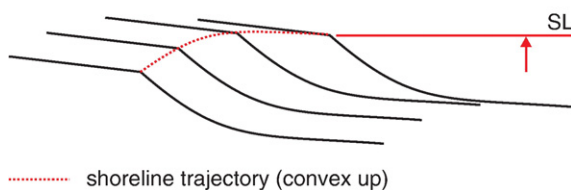
Fig. 18. Stratal stacking patterns of 'lowstand' and 'highstand' normal regressions (modified from Catuneanu, 2006). In both cases progradation is driven by sediment supply: sedimentation rates outpace the rates of base-level rise at the shoreline. Lowstand normal regressions record a change in depositional trends from dominantly progradational to dominantly aggradational (concave up shoreline trajectory). In contrast, highstand normal regressions record a change from aggradation to progradation (convex up shoreline trajectory). These depositional trends reflect the pattern of change in the rates of creation of accommodation during the two types of normal regression (Fig. 16). See Fig. 19 for seismic examples.
