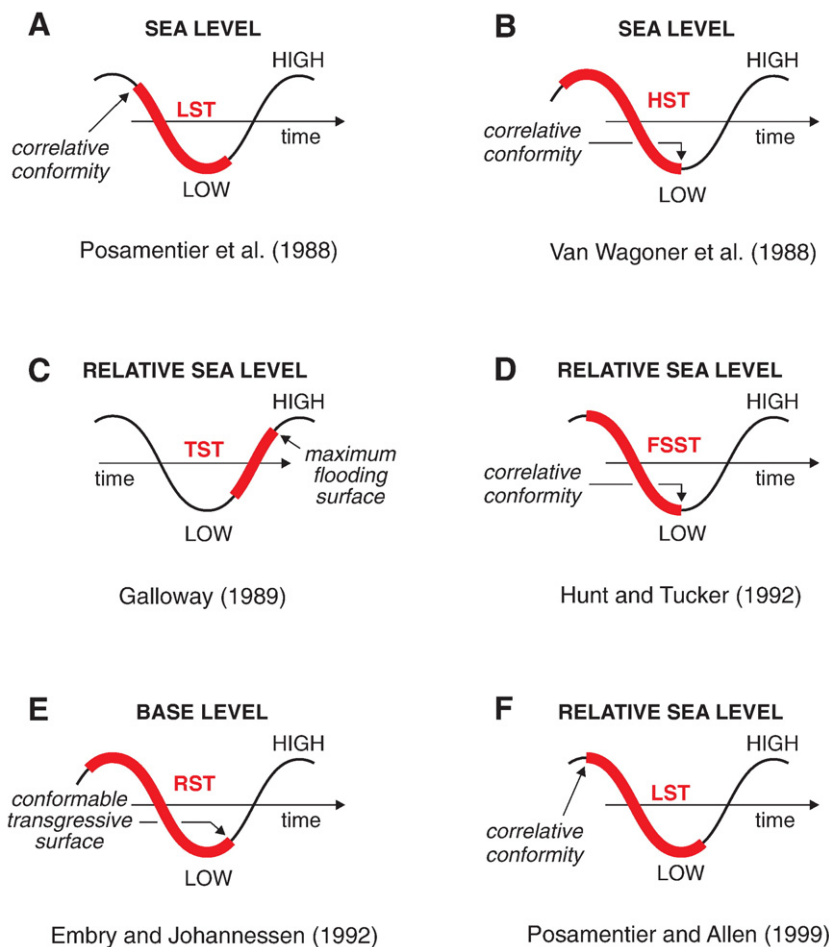
Fig. 23. Correlative conformities as defined by different sequence stratigraphic models (from Catuneanu, 2006). The timing of formation of correlative conformities may be independent of sedimentation (models A, B, D and F), or dependent upon sedimentation (models C and E). Each correlative conformity shown in this diagram corresponds to a particular type of stratigraphic surface shown in Fig. 15: the correlative conformity sensu Posamentier et al. (1988) and Posamentier and Allen (1999) (models A and F); the correlative conformity sensu Hunt and Tucker (1992) (models B and D); the 'maximum flooding surface' (model C); and the 'maximum regressive surface' (model E). The thicker portion of the reference sine curve in each diagram represents the timing of formation of particular systems tracts considered in those models (see abbreviations). Abbreviations: LST – lowstand systems tract; HST – highstand systems tract; TST – transgressive systems tract; FSST – falling-stage systems tract; RST – regressive systems tract.
