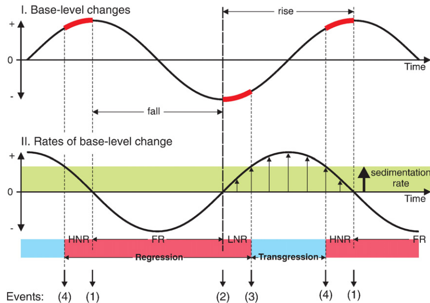
Fig. 16. Concepts of transgression, normal regression, and forced regression, as defined by the interplay of base-level changes and sedimentation at the shoreline (from Catuneanu, 2006). The top sine curve shows the magnitude of base-level changes through time. The thicker portions on this curve indicate early and late stages of base-level rise ('lowstand' and 'highstand' normal regressions respectively), when the rates of base-level rise (increasing from zero and decreasing to zero, respectively) are outpaced by sedimentation rates. The sine curve below shows the rates of base-level changes. Note that the rates of base-level change are zero at the end of base-level rise and base-level fall stages (the change from rise to fall and from fall to rise requires the motion to cease). The rates of base-level change are the highest at the inflection points on the top curve. Transgressions occur when the rates of base-level rise outpace the sedimentation rates. For simplicity, the sedimentation rates are kept constant during the cycle of base-level shifts. The reference base-level curve is shown as a symmetrical sine curve for simplicity, but no inference is made that this should be the case in the geological record. In fact, asymmetrical shapes are more likely (e.g., glacio-eustatic cycles are strongly asymmetrical, as ice melts quicker than it builds up), but this does not change the fundamental principles illustrated in this diagram. Abbreviations: FR – forced regression; LNR – lowstand normal regression; HNR – highstand normal regression. The four events of the base-level cycle are the same as the ones illustrated in Fig. 15: (1) – onset of forced regression; (2) – end of forced regression; (3) – end of regression; (4) – end of transgression.
