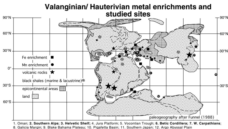
Fig. 2. Valanginian/Hauterivian paleogeography (after Funnel 1988) with the spatial distribution of Fe- and Mn enrichments, continental volcanic rocks and black shales. The location of sections discussed in the text is indicated by numbers and sections analysed in this study are shown by bold text.
