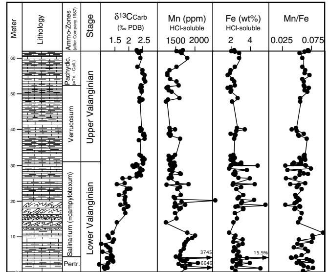
Fig. 7. Section Barranco del Garranchal (Betic Cordillera, southern Spain) with lithologic succession, ammonite zonation (after Company 1987), \delta^{13}\text{C} -curve, contents of Mn and Fe bound in the soluble fraction and Mn/Fe-ratios calculated from these values (after Kuhn 1996). Lithologic key as in Fig. 3.
