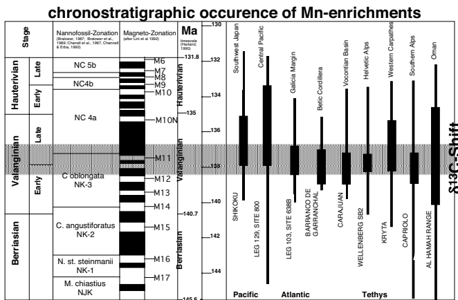
Fig. 8. Chronostratigraphic occurrence of Mn-enrichment levels in the Pacific, Atlantic and the Tethys. The grey bar marks the stratigraphic position of the positive \delta^{13}\text{C} -shift described by Lini et al. (1992), which is interpreted as evidence of a major perturbation of the global carbon cycle.
