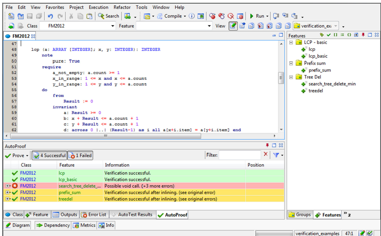
Fig. 1 Screenshot of the EVE IDE integrating AutoProof. The bottom pane shows a verification report for the code in the top pane (discussed in Sect. 3). The first two features (in green) are successfully verified; the third feature (in red) failed verification; the fourth and fifth fea-
