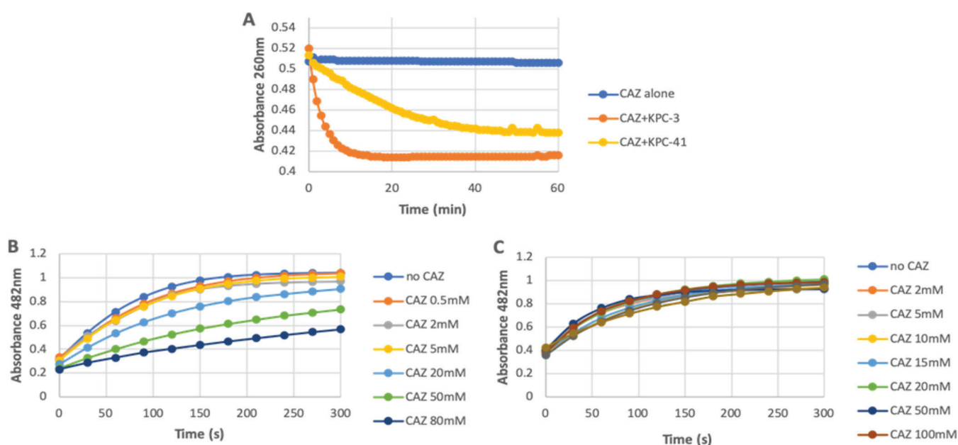
FIG 2 Analysis of ceftazidime hydrolysis. (A) KPC-41 and KPC-3 (1 \mu M enzyme) hydrolysis of 25 \mu M ceftazidime (CAZ) at room temperature. (B and C) Competitive inhibition curves determined with 50 \mu M nitrocefin and increasing concentrations of CAZ with 0.1 \mu M KPC-41(B) and 0.1 \mu M KPC-3 (C) at room temperature. For panels B and C, nitrocefin absorbance was measured.
