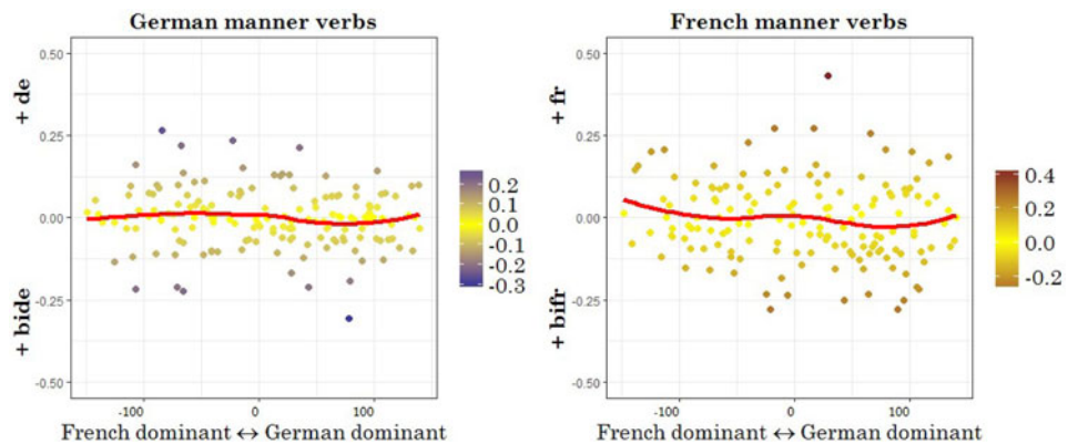
Fig. 3. Mode differences across the dominance scale for manner verbs. Bide refers to the German bilingual mode, de to the German monolingual mode, bifr to the French bilingual mode, fr to the French monolingual mode.
