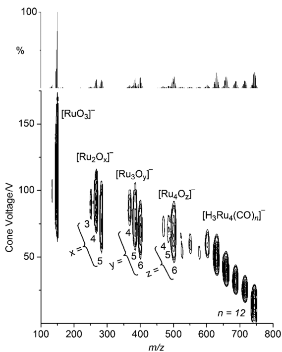
Fig. 11: EDESI-MS of the reaction of [\text{H}_3\text{Ru}_4(\text{CO})_n]^- ( n = 0-12 ) with \text{O}_2(\text{g}) . Adapted from reference [45].
