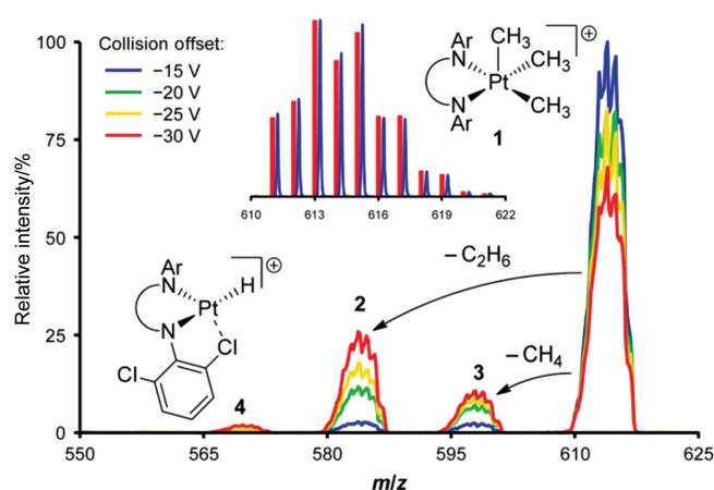
Fig. 14: TCID of [(\text{NN})\text{Pt}^{\text{IV}}\text{Me}_3]^+ ( \text{NN} = \alpha -diimine). Note that the MS signals shown here are much broader than those for standard MS spectra. This is to ensure that the energy of the ions is not unintentionally raised by the isolation process. Reprinted with permission from reference [51]. Copyright 2014 American Chemical Society.
