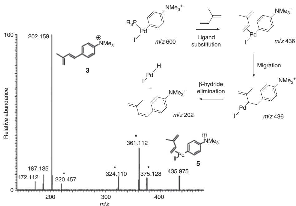
Fig. 9: LTO-MS 3 product ion spectrum of isoprene adduct ion of m/z 436. Reprinted with permission from reference [36]. Copyright © 2011 Elsevier.
