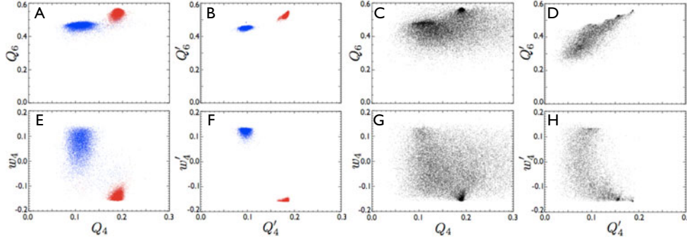
Fig. 2. Comparison of the Q_4 -, Q_6 -, and w_4 -distributions and their averages over nearest neighbors for (A, B, E, F) simulations of fcc and hcp at \phi = 0.28 and for (C, D, G, H) a measurement at \phi = 0.28 .
