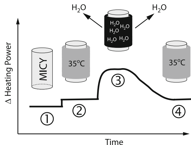
Fig. 4 Graphical scheme of experimental procedure (time progression versus \Delta heating power to maintain cylinder temperature at 35^\circ\text{C} is displayed) using mini cylinder test device MICY. Labels 1 MICY only, 2 laminate sample wrapped around MICY (acclimatization phase), 3 laminate filled with water, evaporation started, 4 end of experiment, all water evaporated
