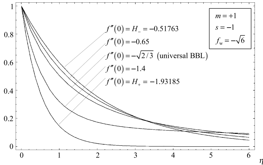
Figure 3. Shape of the dimensionless downstream velocity and temperature profiles f'(\eta) = \vartheta(\eta) of the multiple BBL's for m = 1 and f_w = -\sqrt{6} , and five different values of f''(0) = H(f_w) .
