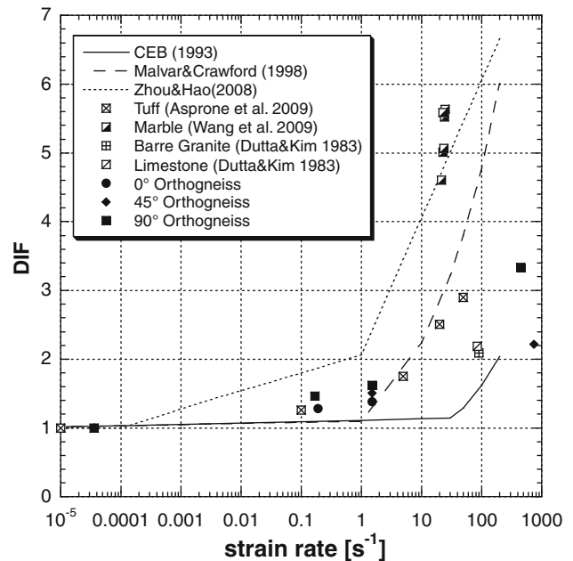
Fig. 9 DIF versus strain rate for different rocks
