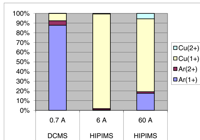
Fig. 5 Ar ion composition and Cu ion composition determined mass spectrometry in the gas phase of a DCMS and a HIPIMS sputtering chamber. For other details, see text
