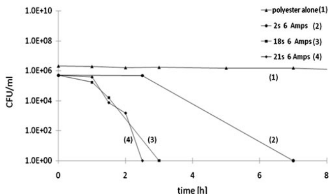
Fig. 3 Kinetics of the E. coli inactivation in the dark by HIPIMS Cu-deposited samples using 6 amps
