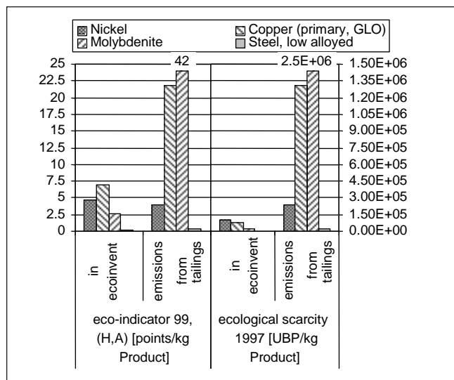
Fig. 1: Impacts from metal production in ecoinvent (neglecting emissions from sulphidic tailings deposition) and from crudely modelled emissions from the deposition of the sulphidic tailings of this production
