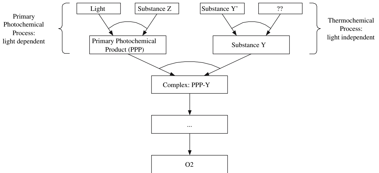
Fig. 6 Expanded model of Warburg’s interpretation of the light curve: whereas the PPP is formed during a light-dependent process, the substance Y is produced during a light-independent series of
