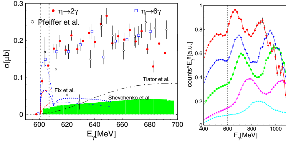
Fig. 22. Left hand side: preliminary total cross section for the \gamma^3\text{He} \rightarrow {}^3\text{He}\eta reaction from \eta \rightarrow 2\gamma and \eta \rightarrow 6\gamma decays [180]. The shaded band at the bottom indicates the systematic uncertainty. The two vertical lines indicate coherent and breakup threshold. Previous data from Pfeiffer et al. [96]. Theory curves: (blue) dotted and dashed from Shevchenko et al. [181] for two different versions of elastic \eta N scattering, (red) solid (dash-dotted): Fix and Arenhövel [182] full model (plane wave), (black) long dash-dotted: Tiator et al. [183]. Right hand side: excitation functions of \pi^0 - p back-to-back pairs for different ranges of the opening angle \Psi_{\pi p} after removal of the overall energy dependence \propto E_\gamma^{-6} . From top to bottom opening angle ranges of: 165^\circ\text{--}180^\circ , 150^\circ\text{--}165^\circ , 140^\circ\text{--}150^\circ , 130^\circ\text{--}140^\circ , and 120^\circ\text{--}130^\circ . Vertical lines: \eta -production threshold.
