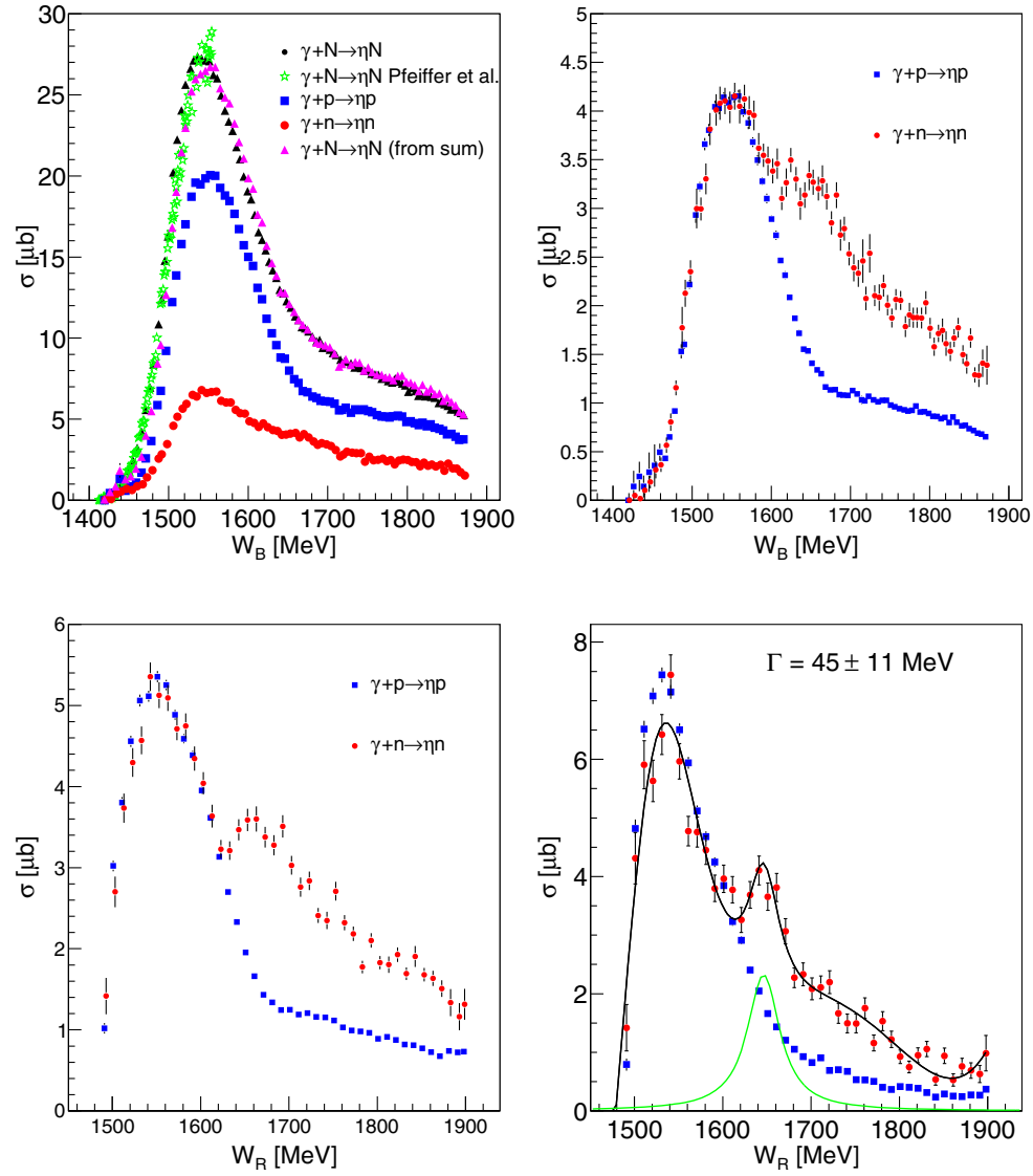
Fig. 17. Preliminary results for quasi-free \eta -photoproduction off ^3\text{He} [150]. Upper left: comparison of quasi-free cross sections off protons and neutrons with inclusive cross section. Previous data for inclusive reaction from Pfeiffer et al. [96]. Upper right: quasi-free proton and neutron cross sections (normalized in S_{11} peak) as function of W from E_\gamma ( W_B ). Lower left: same as function of W reconstructed from final state kinematics ( W_R ) (kinetic energy of neutron from reconstructed kinematics). Lower right: same as function of W_R for kinetic energy of neutron from time-of-flight measurement (only for \eta backward angles).
