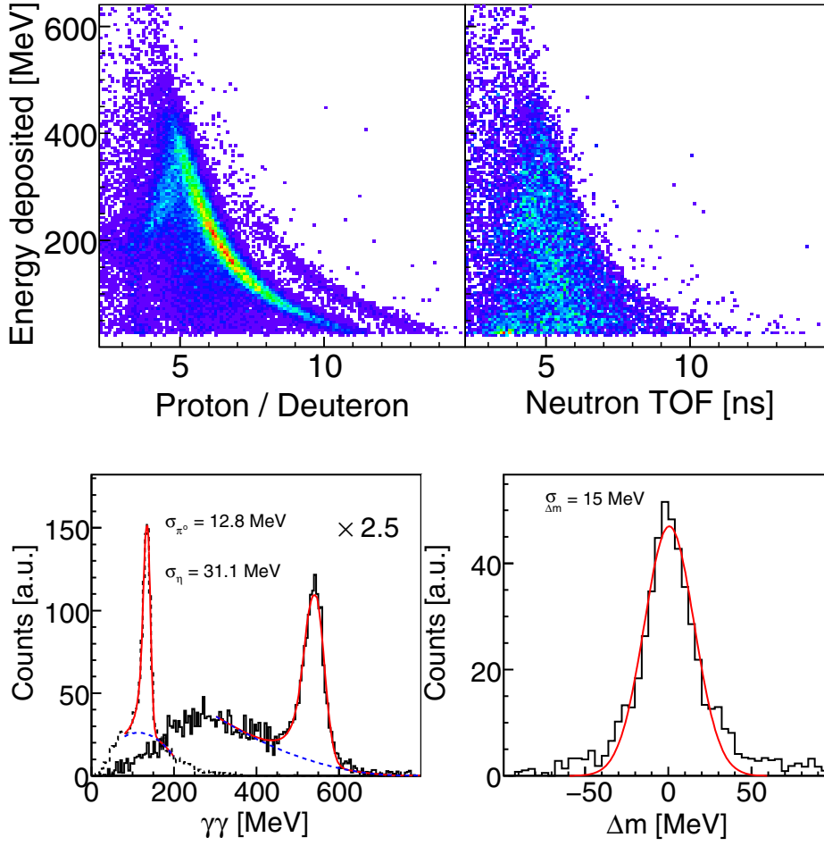
Fig. 20. Identification of the reaction \gamma d \rightarrow d\pi^0\eta [115]. Upper part: time-of-flight versus energy for charged (left hand side) and neutral (right hand side) recoil particles. For the charged particles a prominent band for protons and a weaker band for neutrons is visible. Bottom part: left hand side: invariant mass spectra for \pi^0 and \eta mesons corresponding to the deuteron band in ToF-versus-E. Right hand side: missing mass spectrum after cut on invariant mass.
