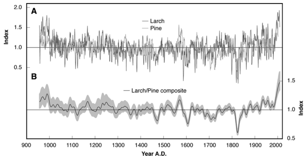
Fig. 4 a Comparison of the RCS detrended larch and pine chronologies since 951, and b the arithmetic mean of these records, smoothed using a 20-year low-pass filter. Shaded envelopes indicate the approximate 95% CI
