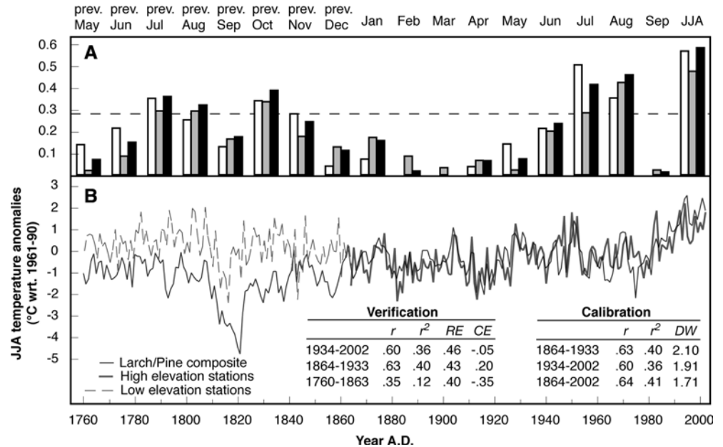
Fig. 6 a Correlations of the RCS detrended pine ( white ) and larch ( grey ) chronologies, and their combination ( black ), with monthly mean temperatures of the previous and current year, calculated over the 1864–1997 common period. The dashed line denotes the 99.9% significance level, corrected for lag-1 autocorrelation. b The RCS larch/pine composite record together with JJA temperatures from high elevation (back to 1864) and low elevation stations (back to 1760). Insert tables show the calibration and verification statistics against JJA temperatures of the current year, with r correlation coefficient, r^2 explained variance, RE reduction of error, CE coefficient of efficiency, and DW Durbin–Watson statistics
