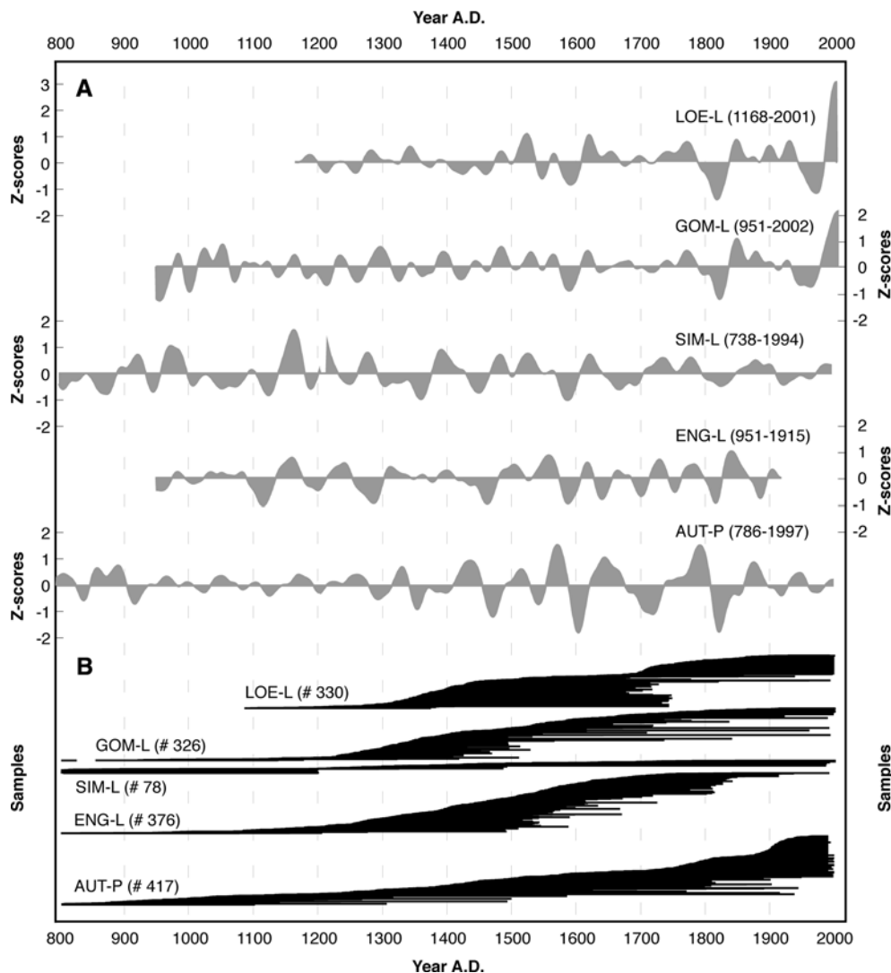
Fig. 2 a Regional ring width chronologies detrended using 300-year spline fittings. Chronologies are truncated at a sample size < 5 series. Numbers in parentheses indicate the length of the records (note the 1201–1211 gap in SIM-L, where sample replication falls below five series). Records smoothed with a 20-year low-pass filter for illustration. b Sample distribution of the chronologies, with each bar representing a single series
