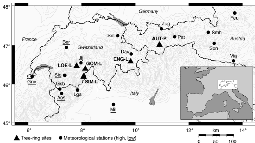
Fig. 1 Locations of 11 high and five low elevation meteorological stations (Böhm et al. 2001), and regional ring width datasets. High elevation stations (>1,500 m a.s.l.): Dav Davos (1901), Feu Feuerkogel (1930), Gsb Gr. St. Bernhard (1818), Jff Jungfrauoch (1933), Lga Lago Gabiet (1928), Pat Patscherkofel (1931), Smh Schmittenhöhe (1880), Snt Säntis (1864), Son Sonnenblick (1887), Via Villacher Alpe (1851), Zug Zugspitze (1901). Low elevation
