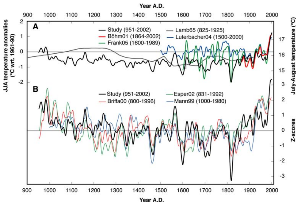
Fig. 7 Comparison of regional and large-scale temperature reconstructions. a The new Alpine RCS detrended record, combining larch and pine data, together with the JJA reconstruction of Frank and Esper (2005b), the JJA reconstruction of Luterbacher et al. (2004) and the reconstruction of Lamb (1965), and the JJA high elevation instrumental temperatures from Böhm et al. (2001). The original records were adjusted to have the same mean during the 1961–1990 period, except for Lamb65, which refers to July–August mean temperatures (see axis on the right). b The Alpine larch/pine
