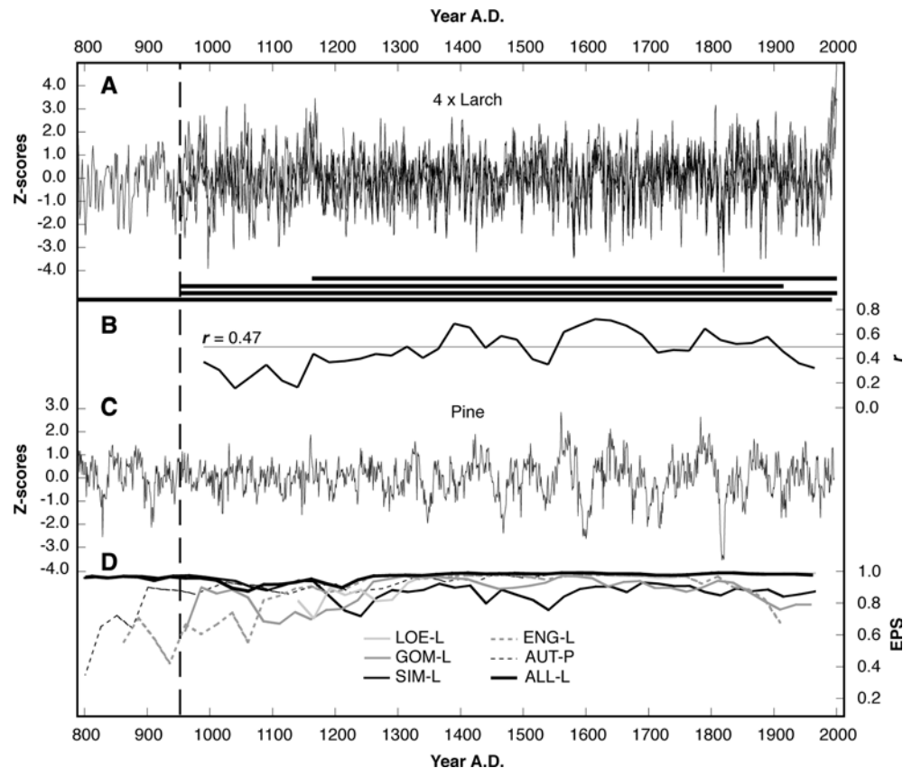
Fig. 3 Three hundred year spline-detrended chronologies and signal strength statistics. a Four larch chronologies and periods covered by these records ( horizontal bars ). B Average cross-chronology correlation r of the four larch records calculated for 50-year periods (offset is 25 years). c Spline-detrended pine chronology. d EPS statistics (Wigley et al. 1984) of the regional site chronologies and a chronology using all larch data, calculated for 50-year periods (offset is 25 years). The vertical dashed line in 951 indicates the period covered by four regional chronologies, with reasonable signal strength statistics in the ALL-L and AUT-P chronologies
