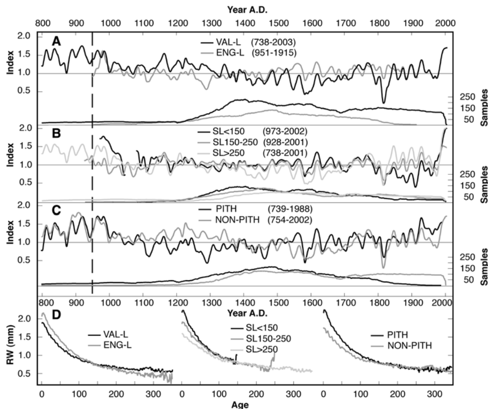
Fig. 5 RCS chronologies derived after splitting the larch data (1110 series) into a the regions ‘Valais’ (734) and ‘Engadine’ (376), b series with segment length < 150 years (614), series with SL 150–250 years (312), series with SL > 250 years (184), and c series including the pith (518) and series with pith offset (396). Sample replications are indicated at the bottom of a–c . d Average growth curves (RC) of the age-aligned data after splitting
