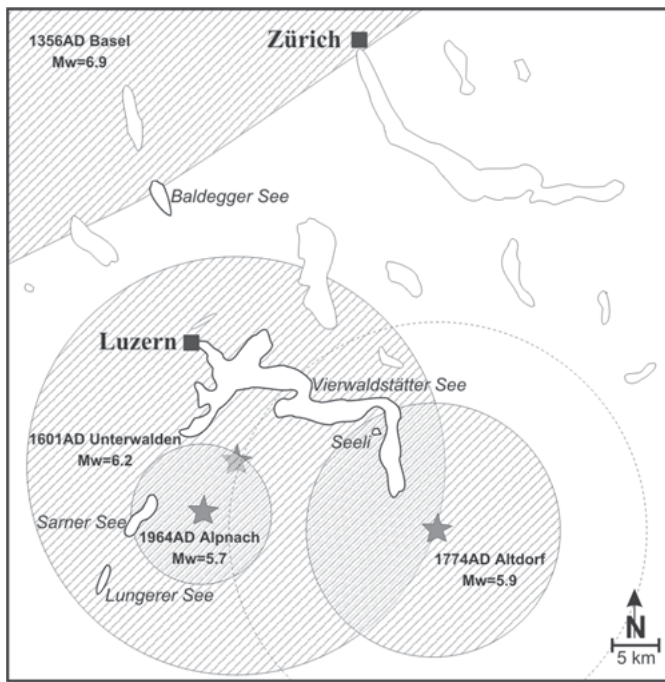
Fig. 17. Areas with expected groundshaking of intensity \geq VII of the four largest historic earthquakes affecting the area of Central Switzerland during the last 1000 years. Dashed line mark area with expected groundshaking of intensity VII of hypothetical M_w = 6.2 event in the Altdorf region (intensity attenuation relation for 1964 Alpnach, 1774 Altdorf and 1601 Unterwalden earthquakes after Swiss Seismological survey, 2002; 1356 Basel earthquake after Mayer-Rosa & Cadiot, 1979).
