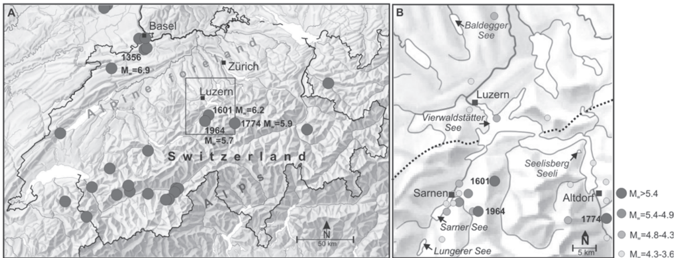
Fig. 1. A) Historic seismicity in Switzerland and surrounding areas. B) Location of studied lakes. Dashed line marks northern Alpine front. Dots mark epicenters of historic earthquakes of the last 1000 years with moment magnitudes M_w > 5.4 (Fig. 1A) and M_w > 3.6 (Fig. 1B; after Fäh et al., 2003).
