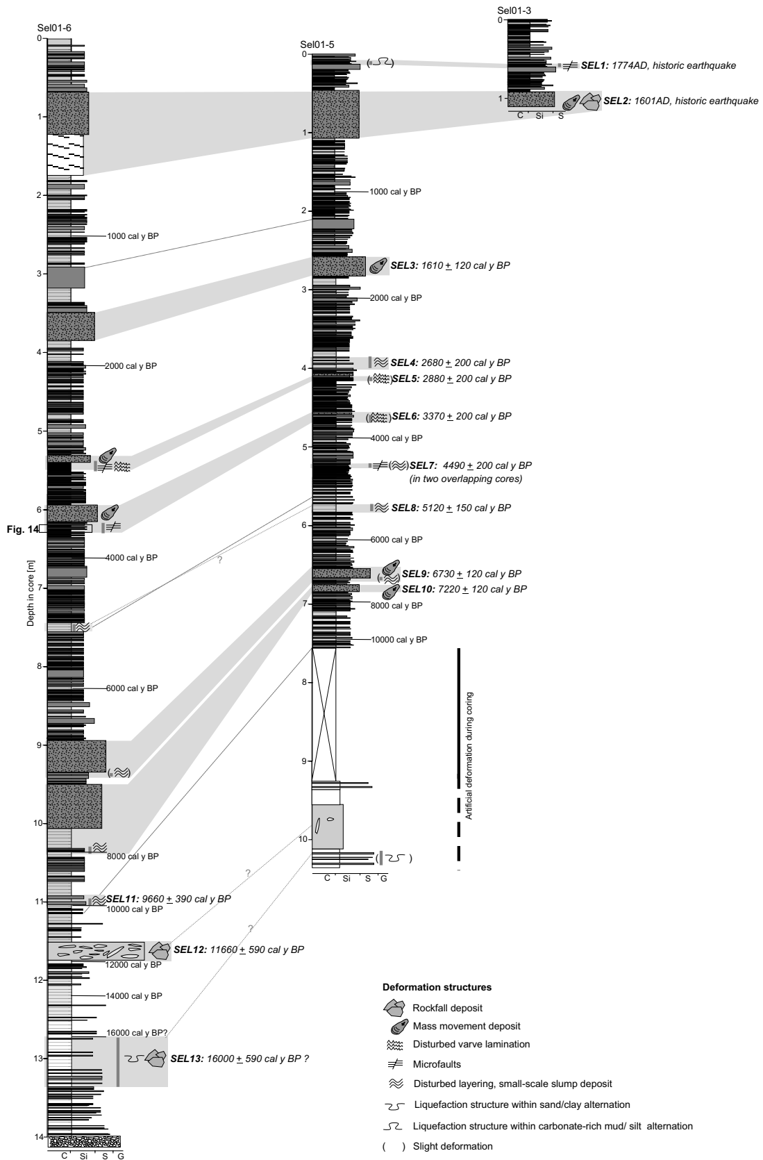
Fig. 13. Core-to-core correlations of events within the sedimentary record of Seelberg Seeli. Lithology legend as in Fig. 4. See Fig. 11 for coring locations.
