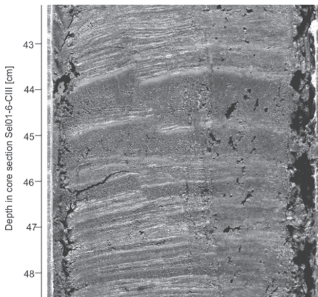
Fig. 14. Microfaults within alternating varves and flood-generated turbidites of Seelisberg Seeli (core section Sel01-6-CIII).
