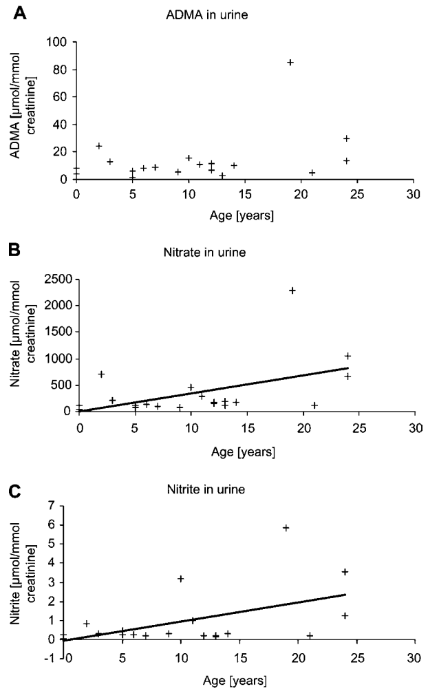
Figure 2 Correlation between urinary creatinine-corrected excretion rate of (A) asymmetric dimethylarginine (ADMA) ( n=20 , r=-0.241 , p>0.05 ), (B) nitrate ( n=20 , r=0.471 , p<0.05 ), or (C) nitrite ( n=20 , r=0.484 , p<0.05 ) and age of healthy infants and young adults.
