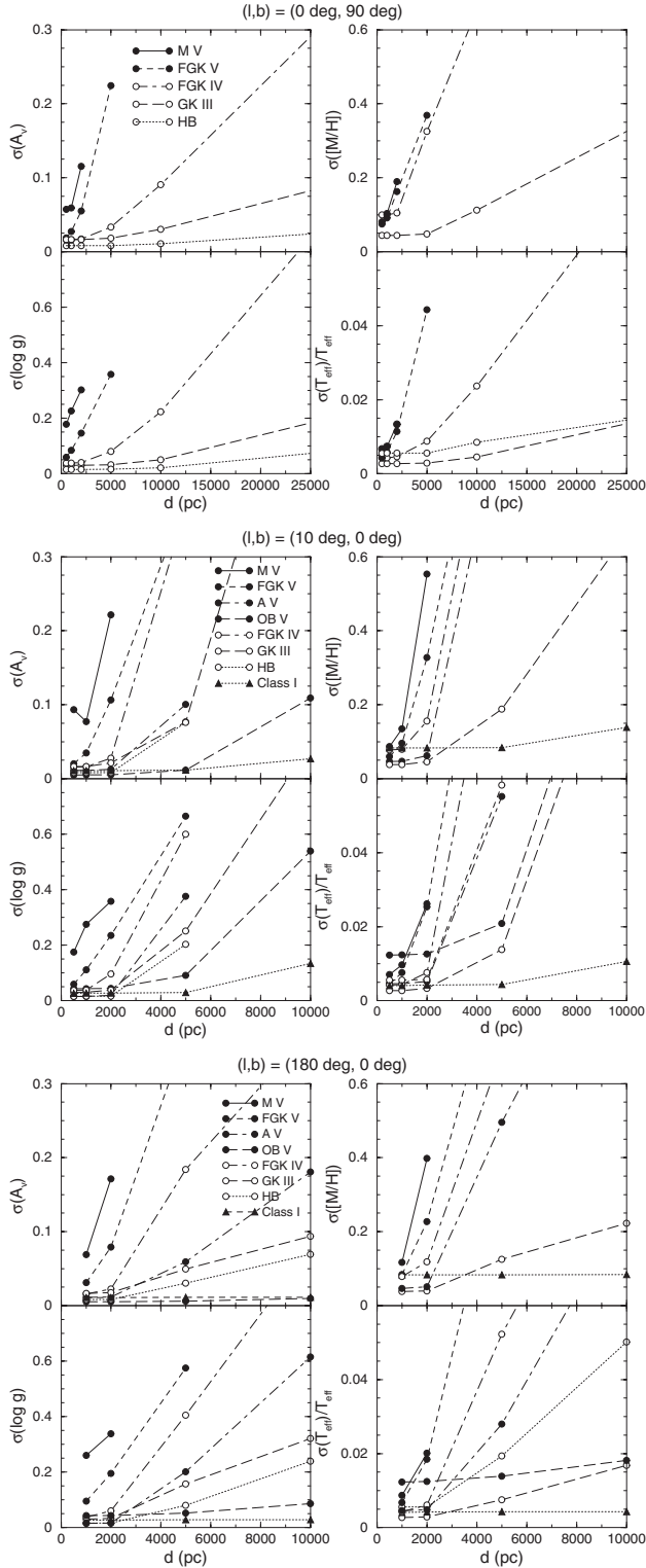
Figure 12. Predicted (posterior) errors for the main astrophysical parameters in three Galactic directions based on G, C1B, C1M and parallax data. The following assumption holds for A_V : in the Galactic pole direction it reaches 0.3 mag at 1 kpc and is constant from this distance onwards; towards the Galactic centre it ranges from 0.3 mag at 500 pc to 10 mag at 10 kpc; and towards the anticentre it varies from 0.3 mag at 500 pc to 3.5 mag at 5 kpc and is constant for large distances. The figure legends indicate the meaning of the lines, where ‘Class I’ means luminosity class I and ‘HB’ means horizontal branch stars.
