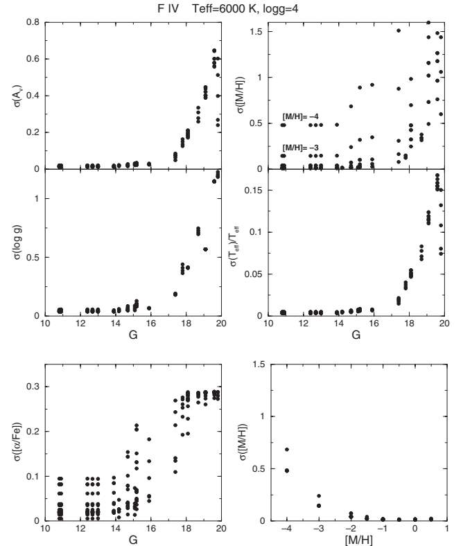
Figure 13. Predicted (posterior) errors for the astrophysical parameters as a function of apparent G magnitude and [M/H] for F-type subgiants. The top four panels show the results based on the BaSeL 2.2 SED library. In the top right panel, the metallicity increases from [M/H] = -4 at the top to [M/H] = +0.5 at the bottom for each vertical set of dots. The bottom left panel shows the predicted errors for [\alpha/\text{Fe}] based on the NEXTGEN 2 SED library. The bottom right panel shows the error on [M/H] as a function of [M/H] for stars brighter than G = 15 (based on BaSeL 2.2 SEDs).
