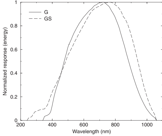
Figure 2. The G and GS Gaia broad passbands corresponding to the white light observations in the Astro and Spectro focal planes, respectively.
