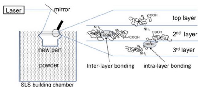
FIG. 12. Interlayer reaction of polyamide 12 during SLS processing.
