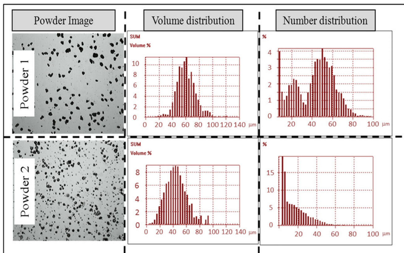
FIG. 4. Distribution of powders with similar volume distribution and dissimilar number distribution.
