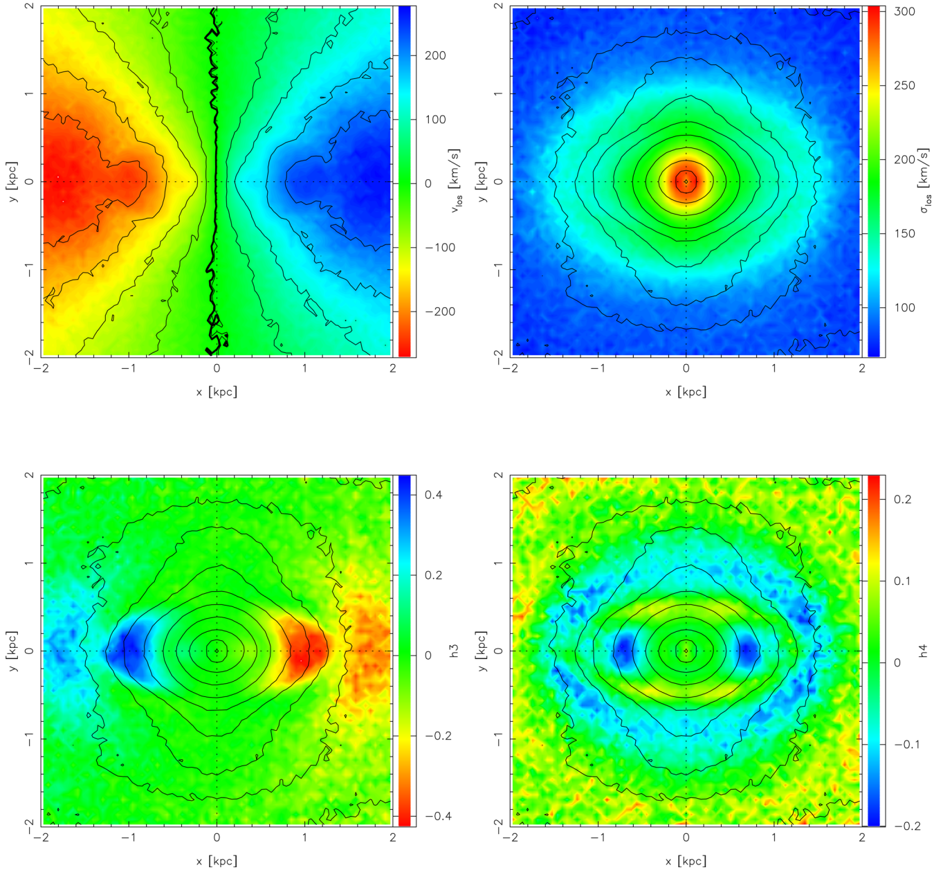
Figure 18. Line-of-sight kinematic maps for the model at 10Gyr projected to the orientation of NGC 3945 (bar PA = 88^\circ , here measured from the x -axis, inclination = 55^\circ ). Top left is v_{\text{los}} , top right is \sigma_{\text{los}} , bottom left is h_3 , bottom right is h_4 . The v_{\text{los}} map shows contours of isovelocity, with the v_{\text{los}} = 0 shown in bold, while the remaining maps show contours of surface density. The bar is nearly vertical in this image, while the ND is almost horizontal.
