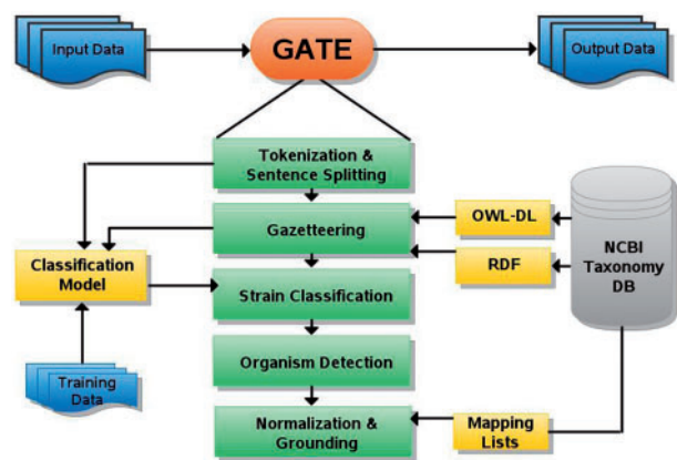
Fig. 1. An overview of the main parts of the OrganismTagger system: document processing is performed by an NLP pipeline running in GATE using resources automatically created from the NCBI Taxonomy database.
