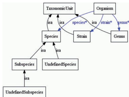
Fig. 2. OWL ontology for organisms: taxonomic units are encoded as OWL classes that can be automatically populated from the NCBI Taxonomy database and then used for automatic semantic annotation of documents.
