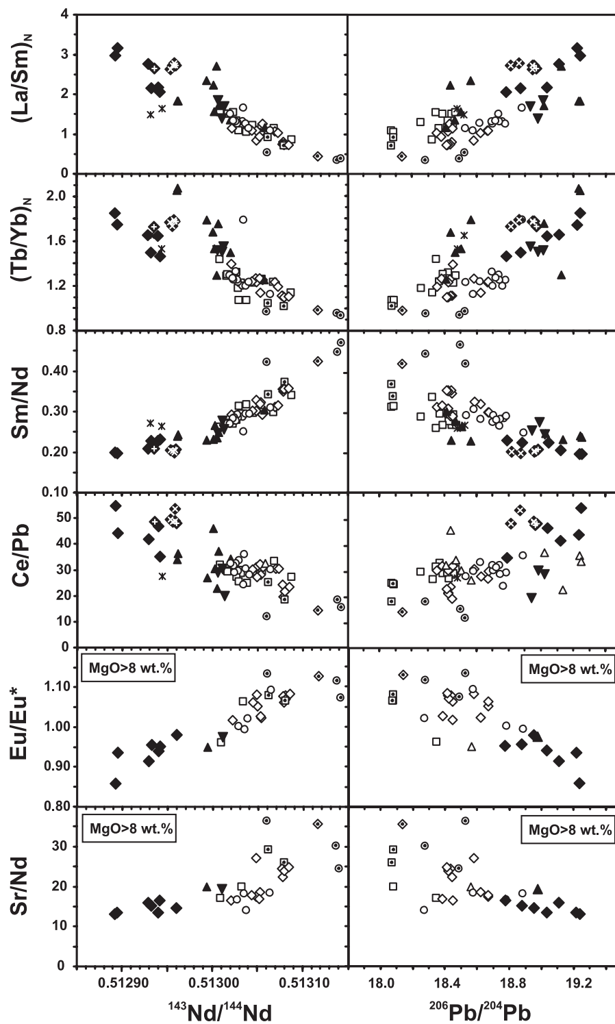
Fig. 9. ^{143}\text{Nd}/^{144}\text{Nd} and ^{206}\text{Pb}/^{204}\text{Pb} vs (\text{La}/\text{Sm})_{\text{N}} , (\text{Tb}/\text{Yb})_{\text{N}} , \text{Sm}/\text{Nd} , \text{Ce}/\text{Pb} , \text{Eu}/\text{Eu}^* and \text{Sr}/\text{Nd} .
