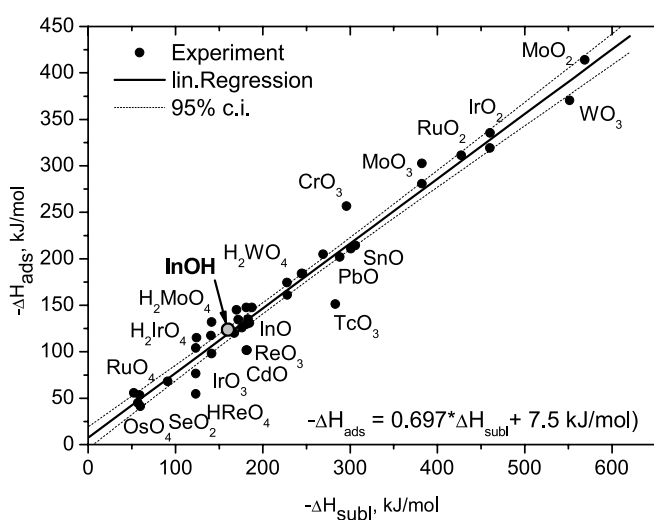
Fig. 8. Correlation of the adsorption enthalpy \Delta H_{\text{ads}} of oxides on quartz surfaces with the macroscopic property sublimation enthalpy \Delta H_{\text{subl}} [22]. The position of InOH within this correlation plot was obtained in this work.
