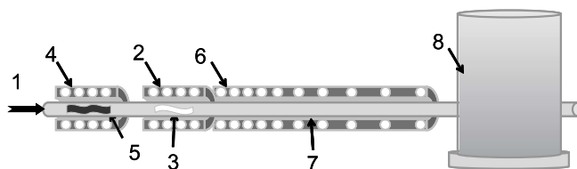
Fig. 3. Thermochromatography set-up. 1 – carrier gas ( \text{Ar} , \text{H}_2 , \text{O}_2 or mixtures with water); 2 – start oven ( 1000/1300^\circ\text{C} ); 3 – ^{113m}\text{In} source either on a tantalum foil, or on a quartz wool surface, or inside of irradiated metallic tin in \text{Al}_2\text{O}_3 ; 4 – getter oven ( 1000^\circ\text{C} ); 5 – Ta chips; 6 – gradient oven; 7 – chromatographic column (quartz/gold), inner diameter 4 mm; 8 – cooling system (up to liquid nitrogen 77\text{ K} temperature).
