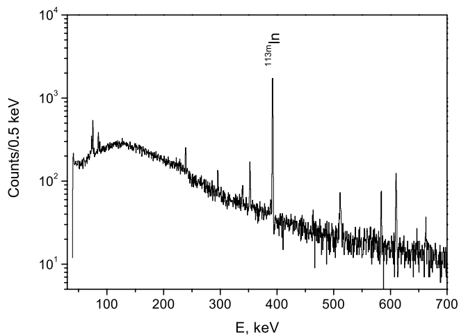
Fig. 2. Gamma spectrum of an eluted ^{113m}\text{In} sample.
